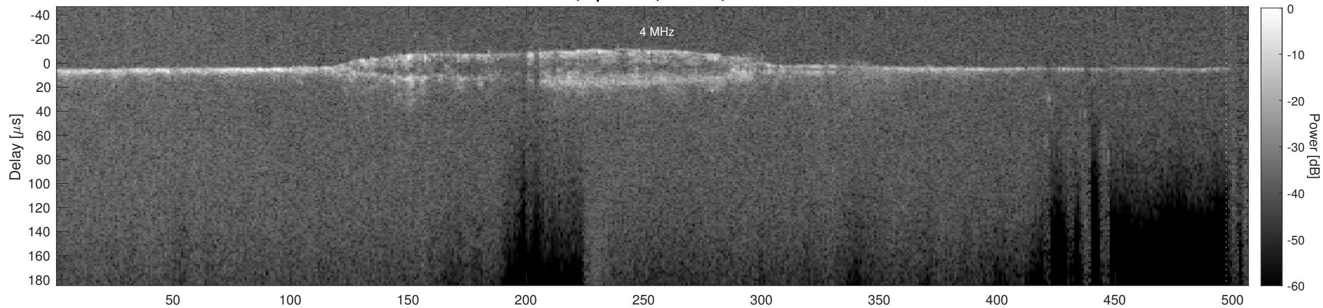
Orbit 5449, Cluttergram
