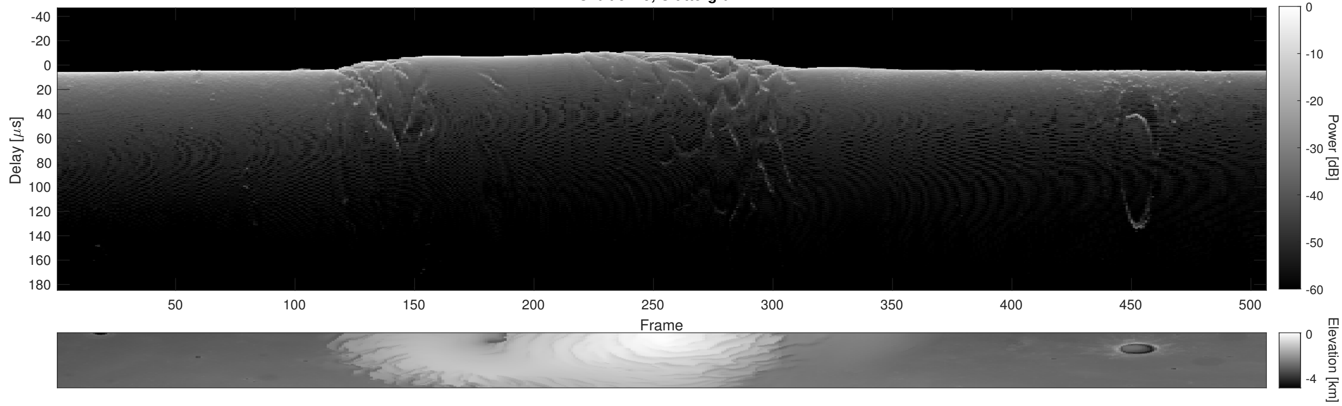
Orbit 5449, Cluttergram
