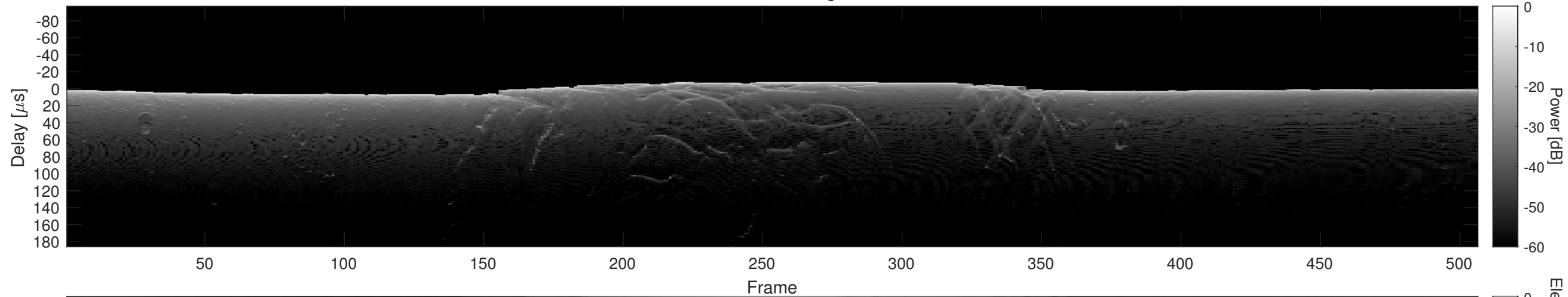
Orbit 5450, Cluttergram
