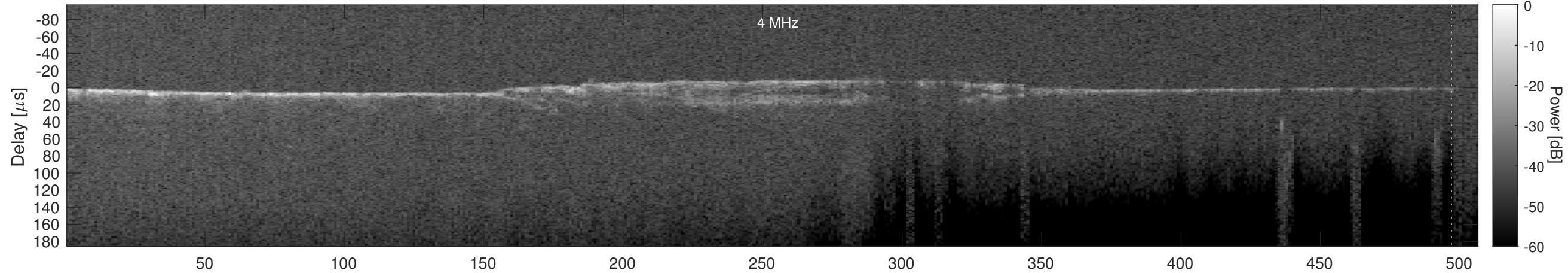
Orbit 5450, Cluttergram
