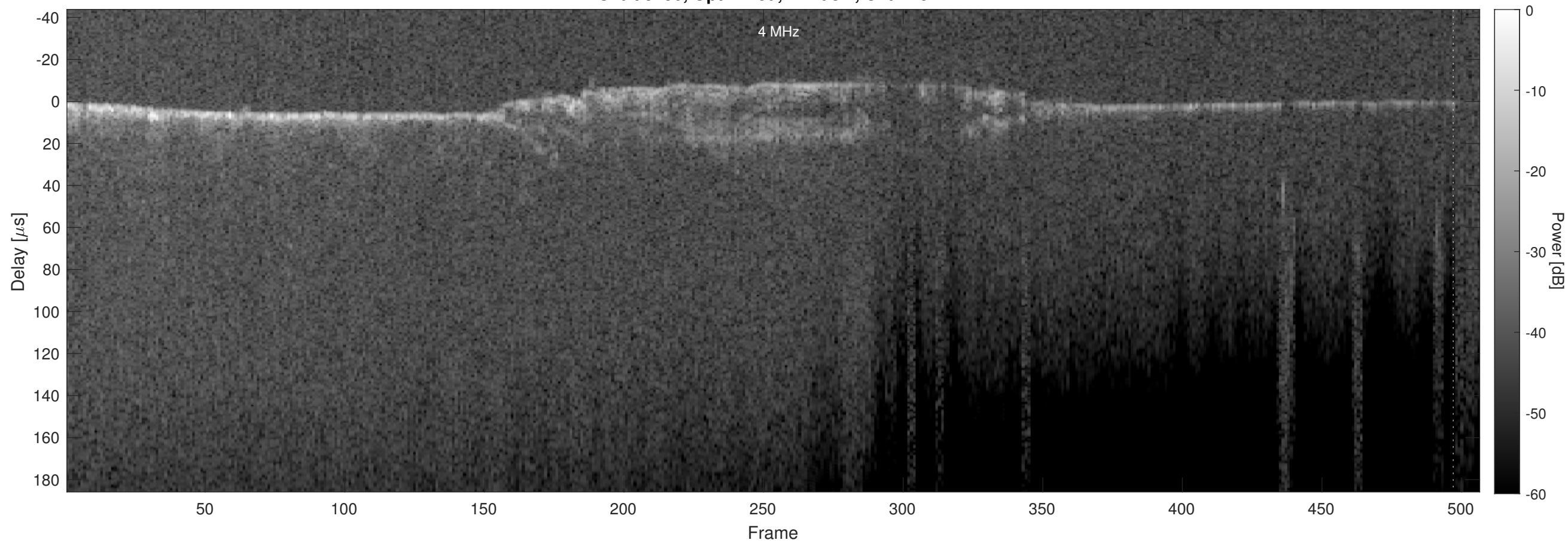
Orbit 5450, Optimized, Window, Channel 2
