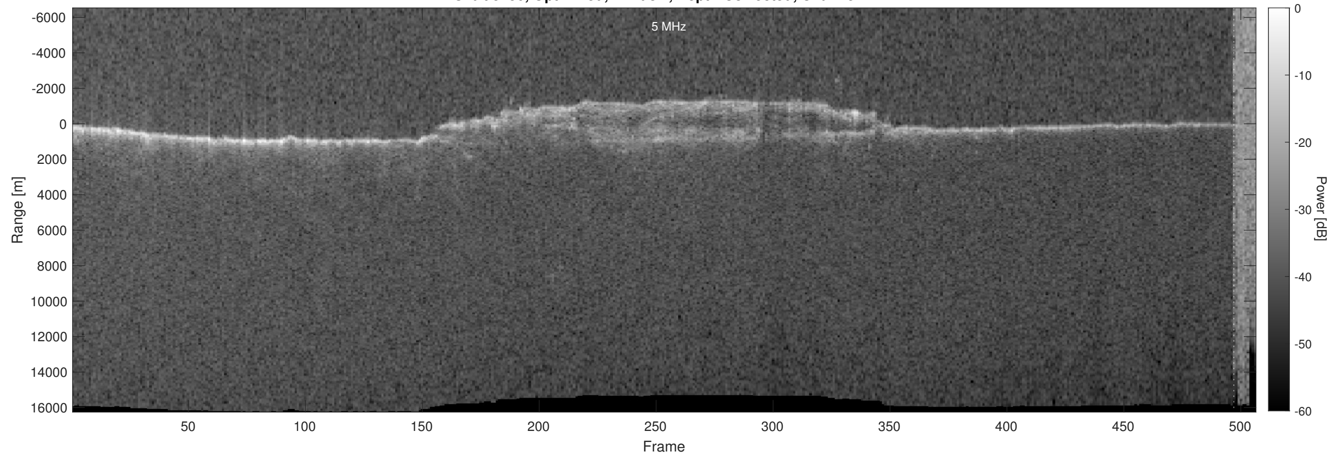
Orbit 5450, Optimized, Window, Depth-Corrected, Channel 2
