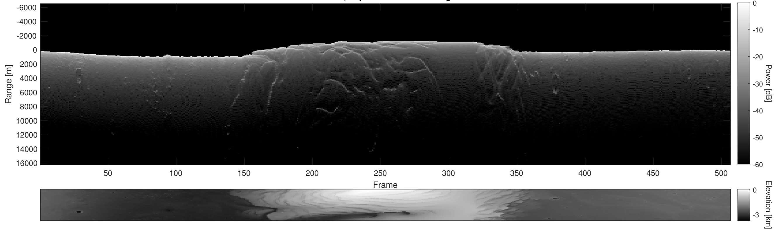
Orbit 5450, Depth-Corrected Cluttergram
