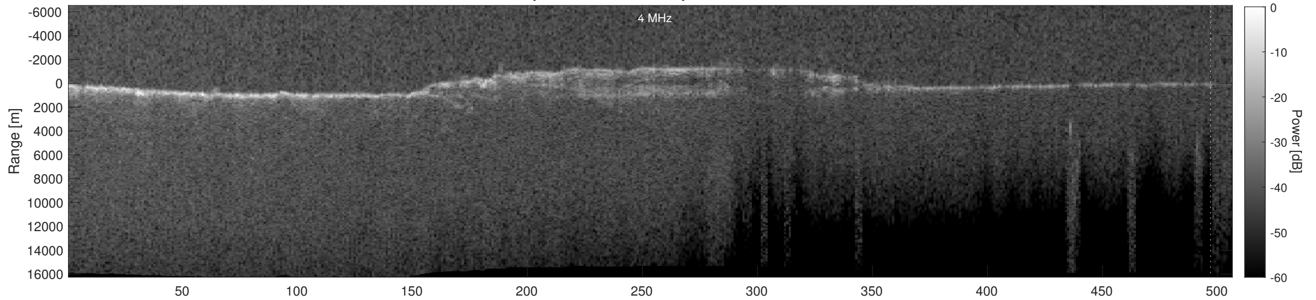
Orbit 5450, Depth-Corrected Cluttergram
