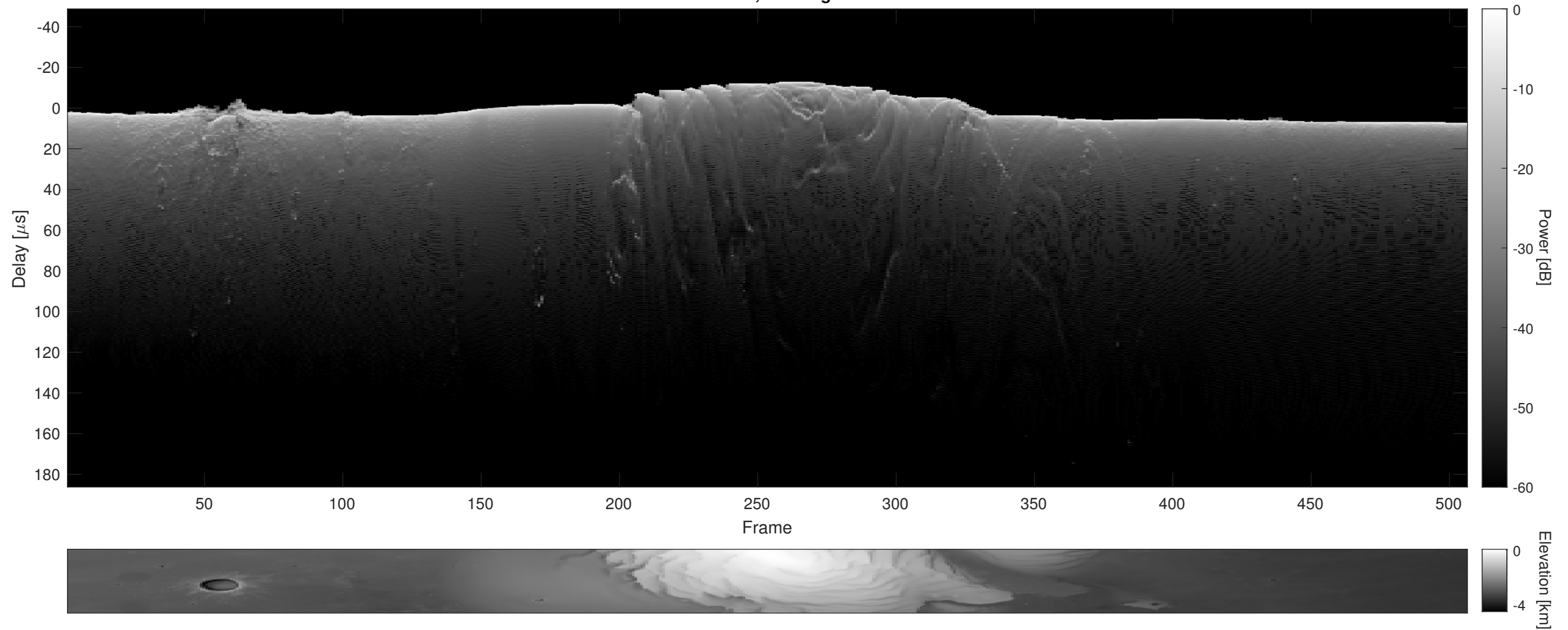
Orbit 5451, Cluttergram
