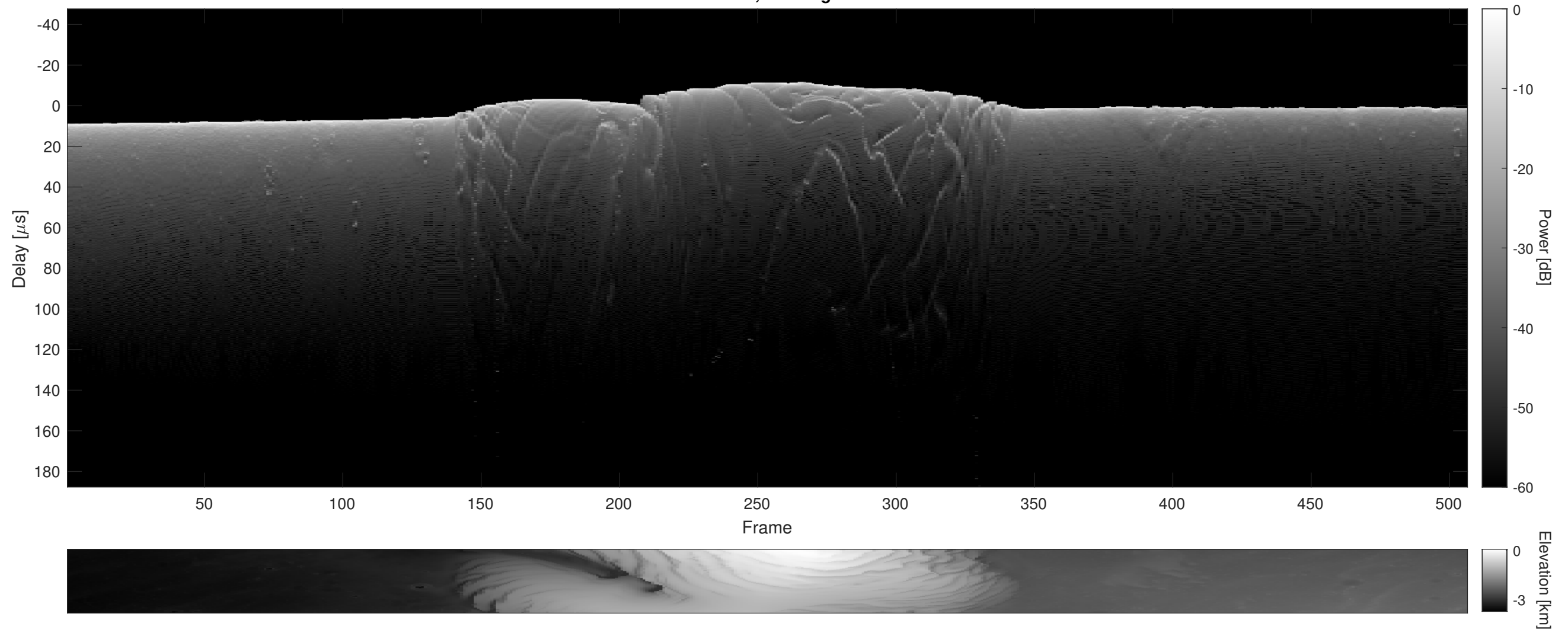
Orbit 5453, Cluttergram
