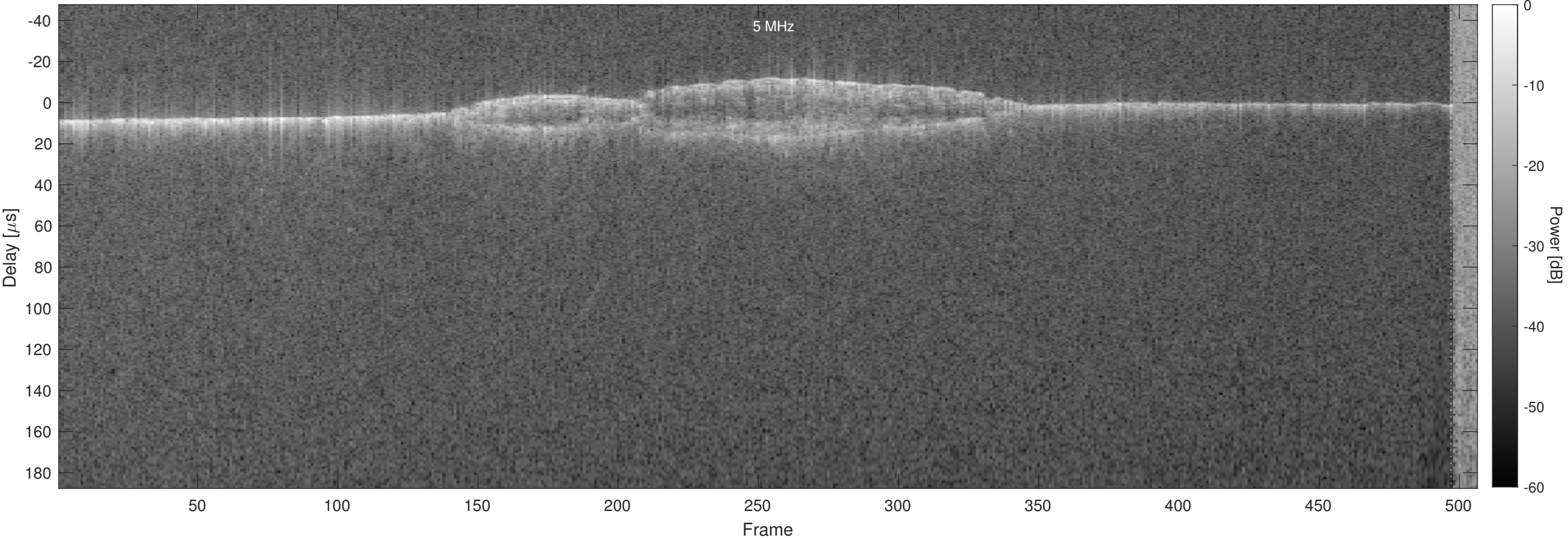
Orbit 5453, Optimized, No Window, Channel 2
