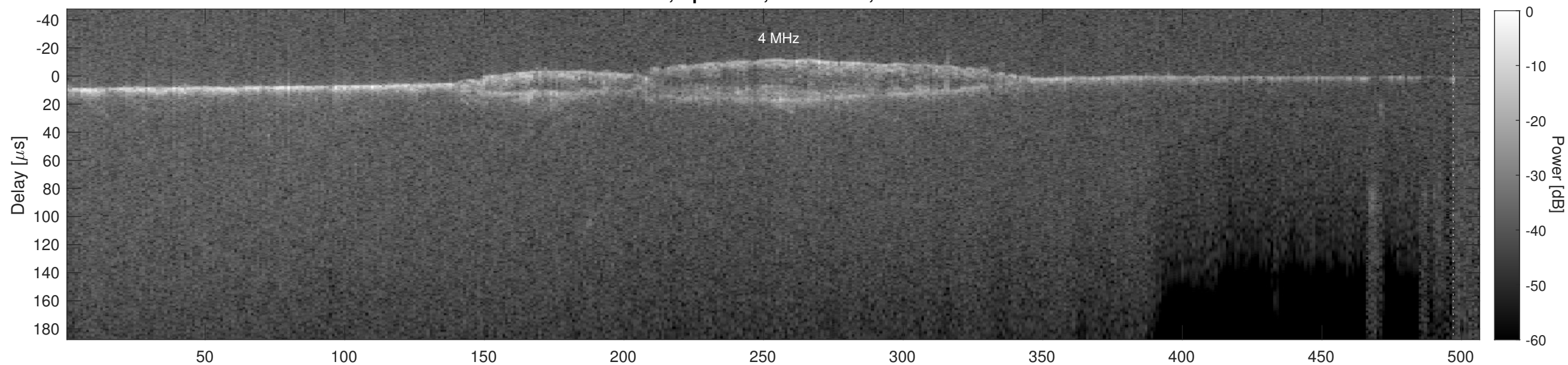
Orbit 5453, Cluttergram
