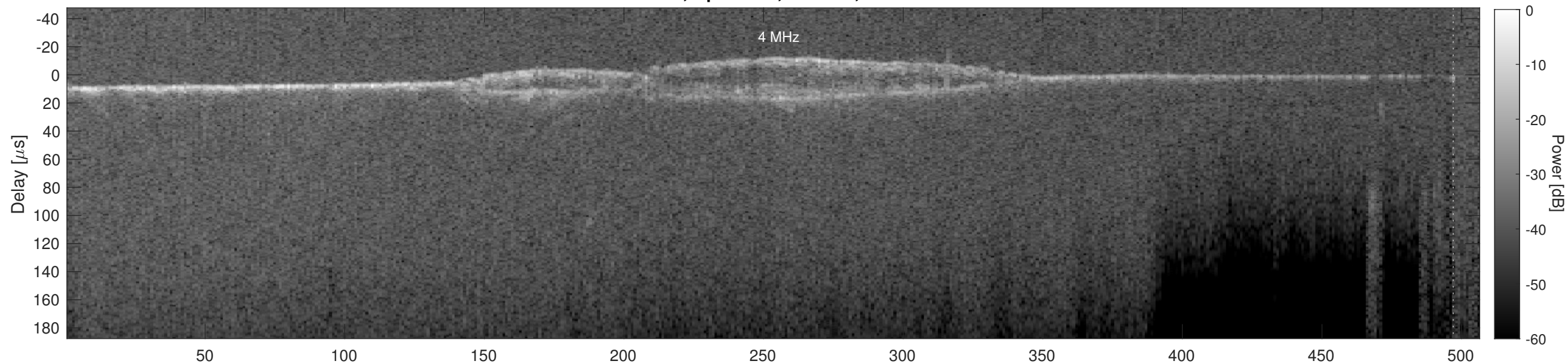
Orbit 5453, Cluttergram
