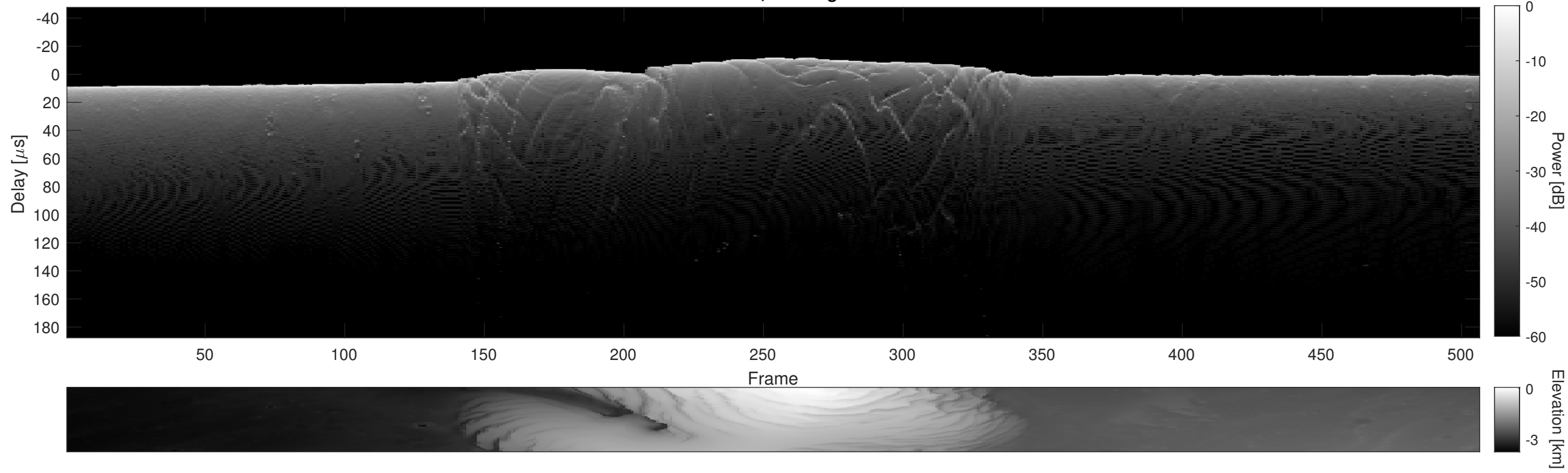
Orbit 5453, Cluttergram
