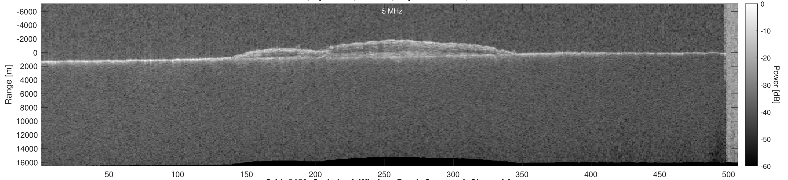
Orbit 5453, Optimized, Window, Depth-Corrected, Channel 2
