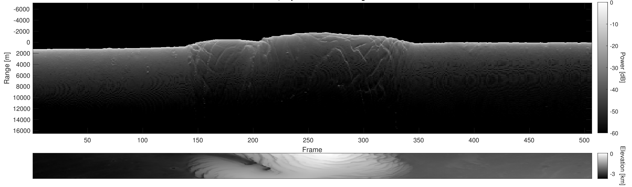
Orbit 5453, Depth-Corrected Cluttergram
