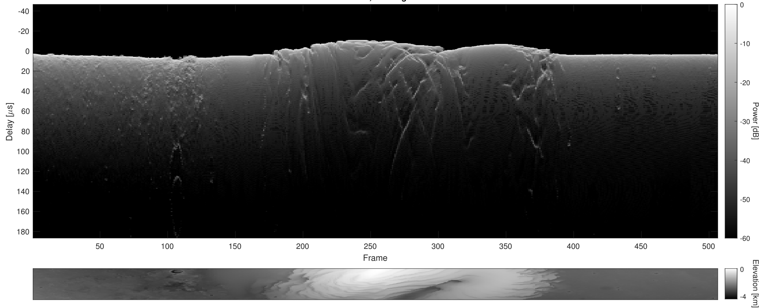
Orbit 5454, Cluttergram
