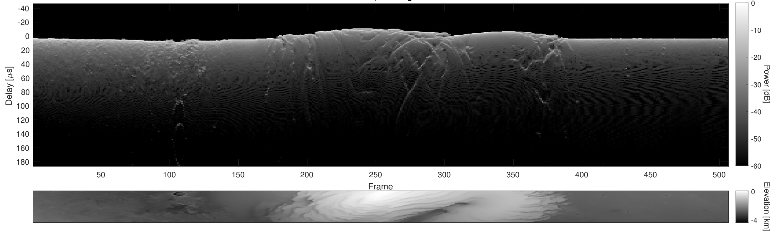
Orbit 5454, Cluttergram
