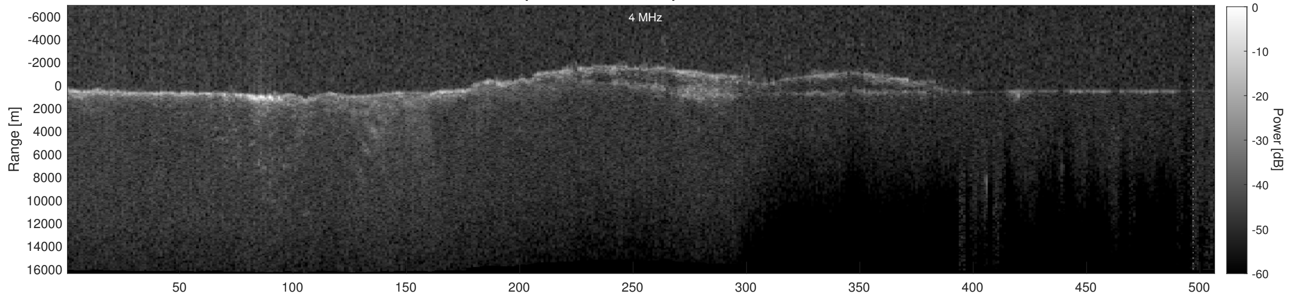
Orbit 5454, Depth-Corrected Cluttergram
