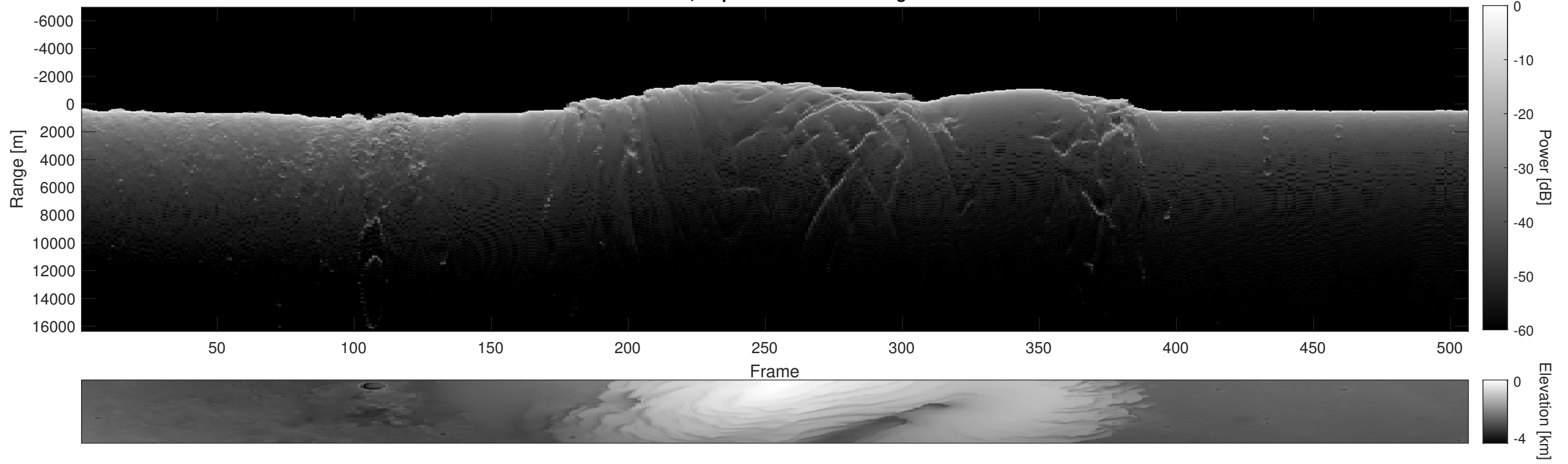
Orbit 5454, Depth-Corrected Cluttergram
