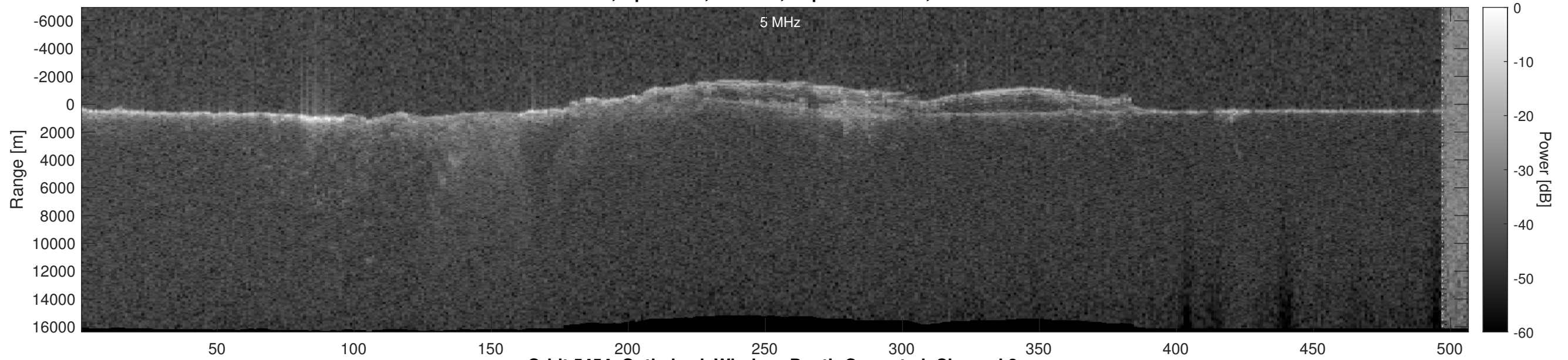
Orbit 5454, Optimized, Window, Depth-Corrected, Channel 2
