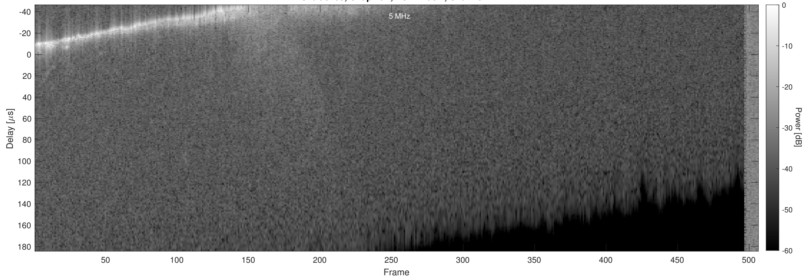
Orbit 5455, Chapman, No Window, Channel 2
