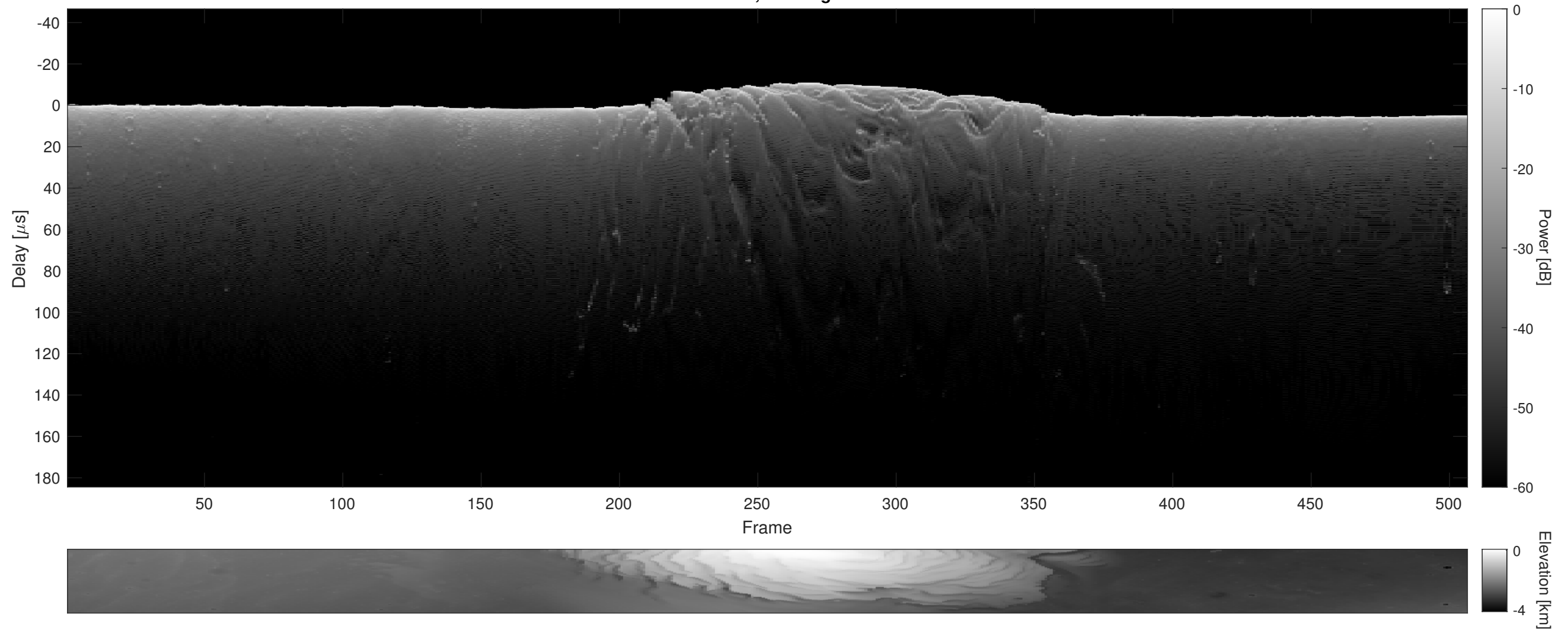
Orbit 5455, Cluttergram
