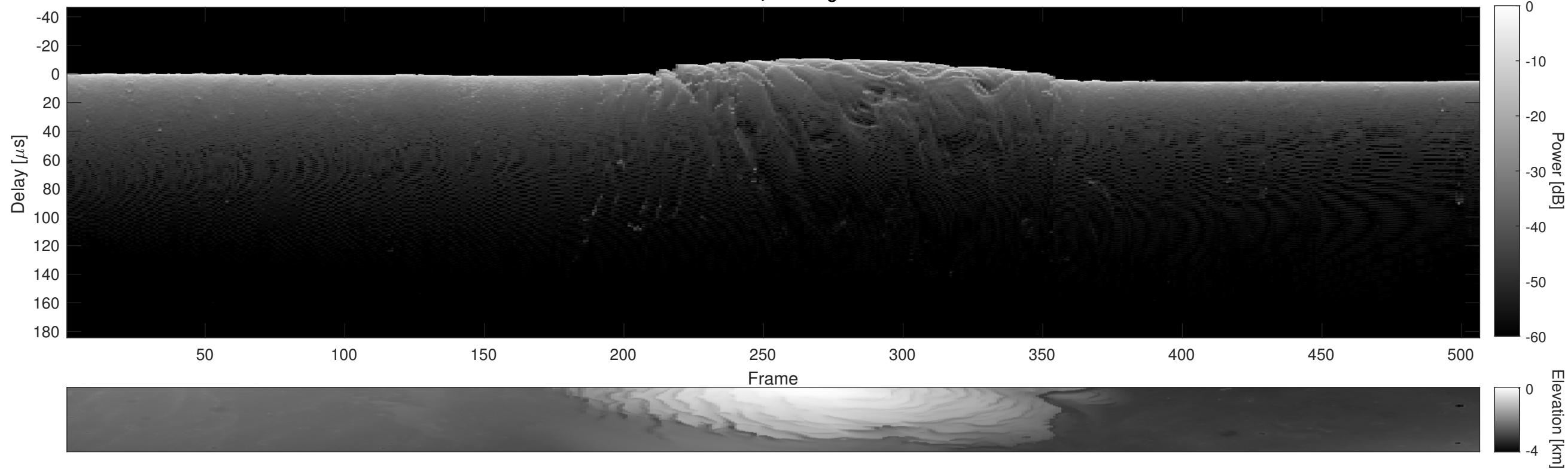
Orbit 5455, Cluttergram
