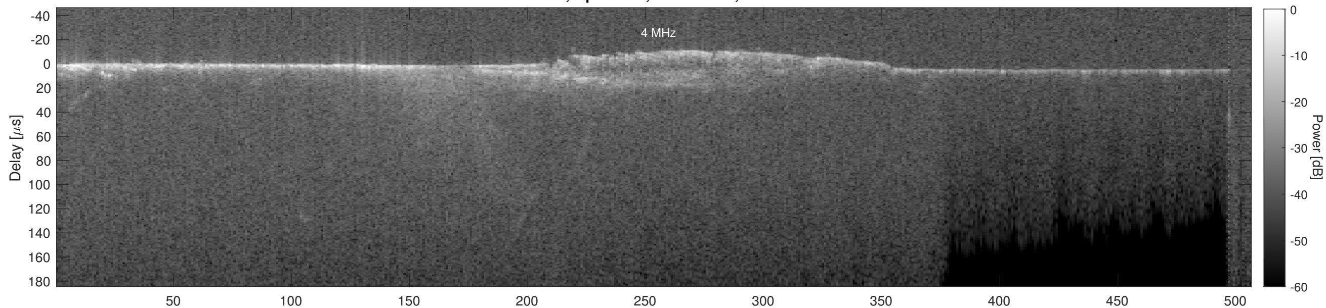
Orbit 5455, Cluttergram
