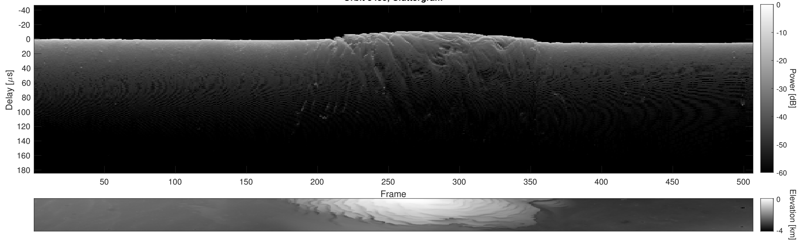
Orbit 5455, Cluttergram
