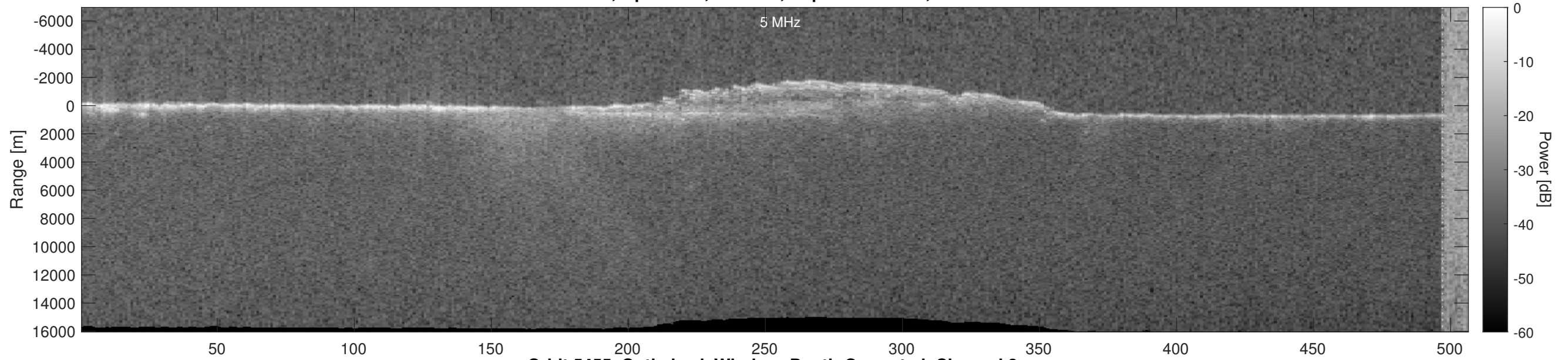
Orbit 5455, Optimized, Window, Depth-Corrected, Channel 2
