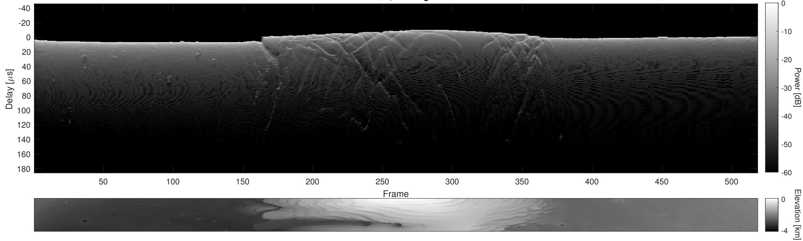
Orbit 5457, Cluttergram
