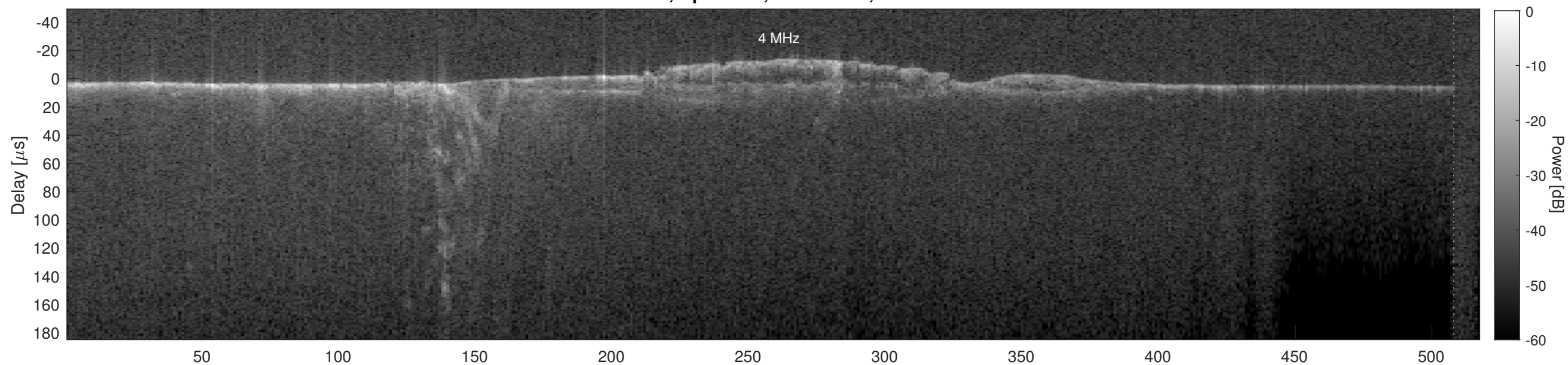
Orbit 5458, Cluttergram
