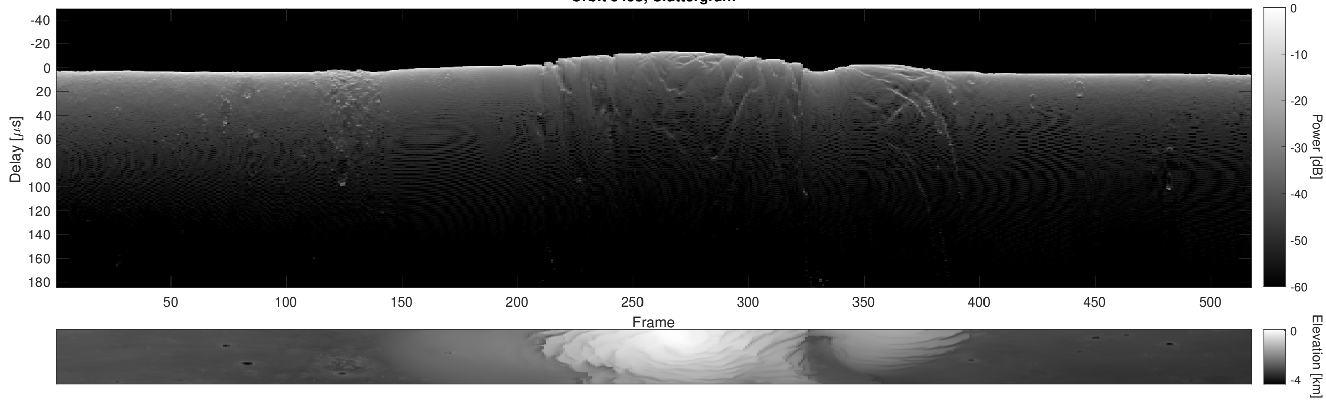
Orbit 5458, Cluttergram
