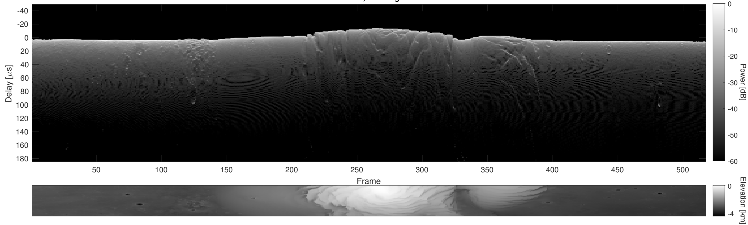
Orbit 5458, Cluttergram
