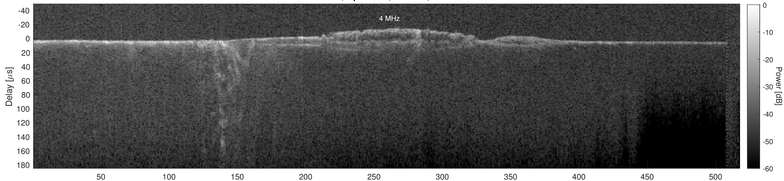
Orbit 5458, Cluttergram
