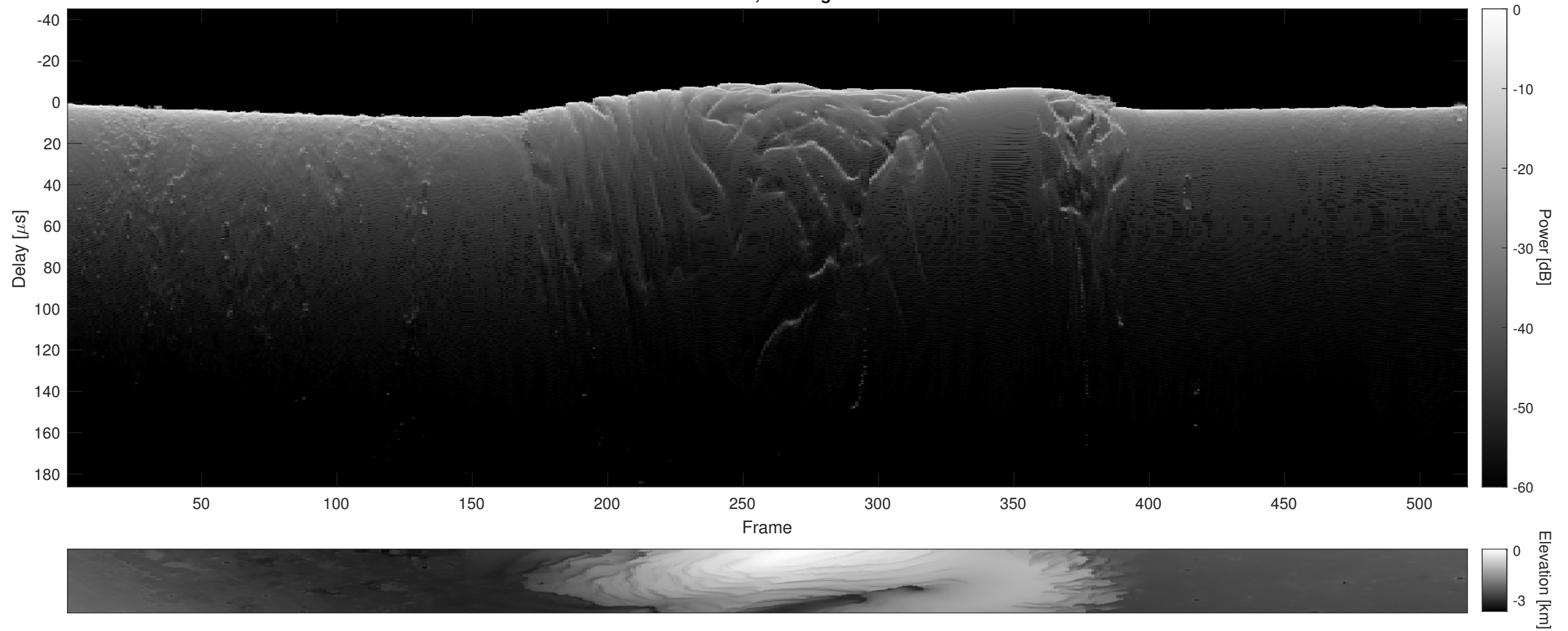
Orbit 5461, Cluttergram
