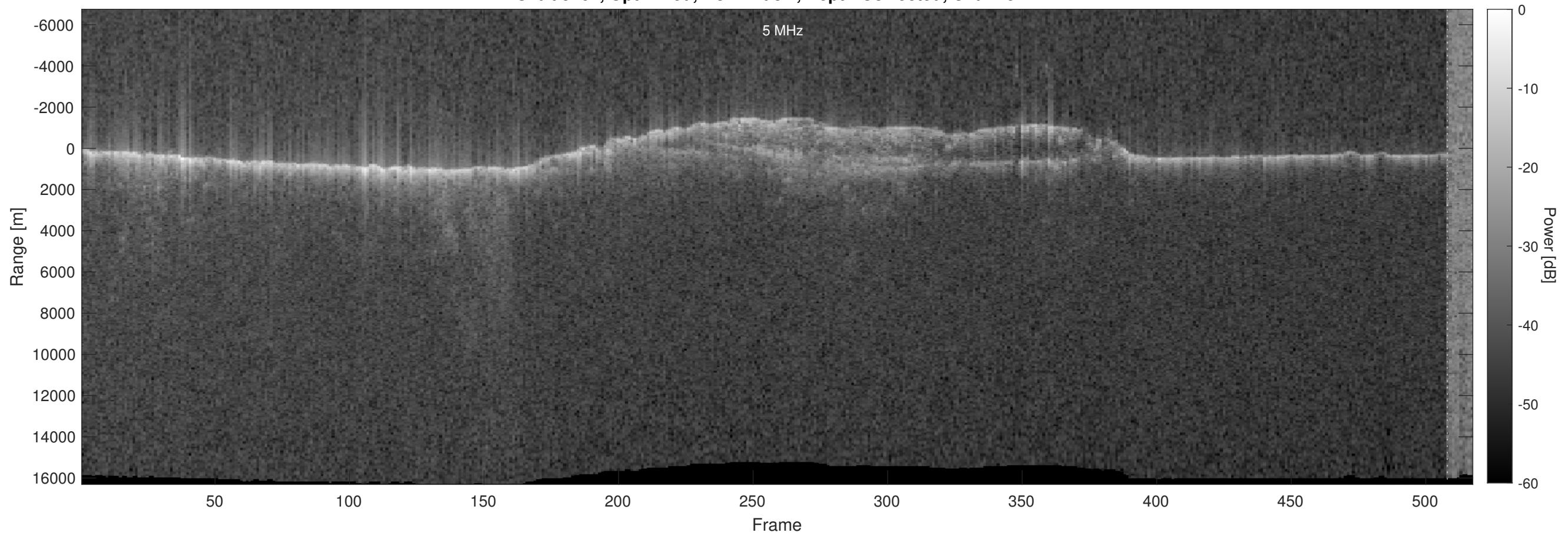
Orbit 5461, Optimized, No Window, Depth-Corrected, Channel 2
