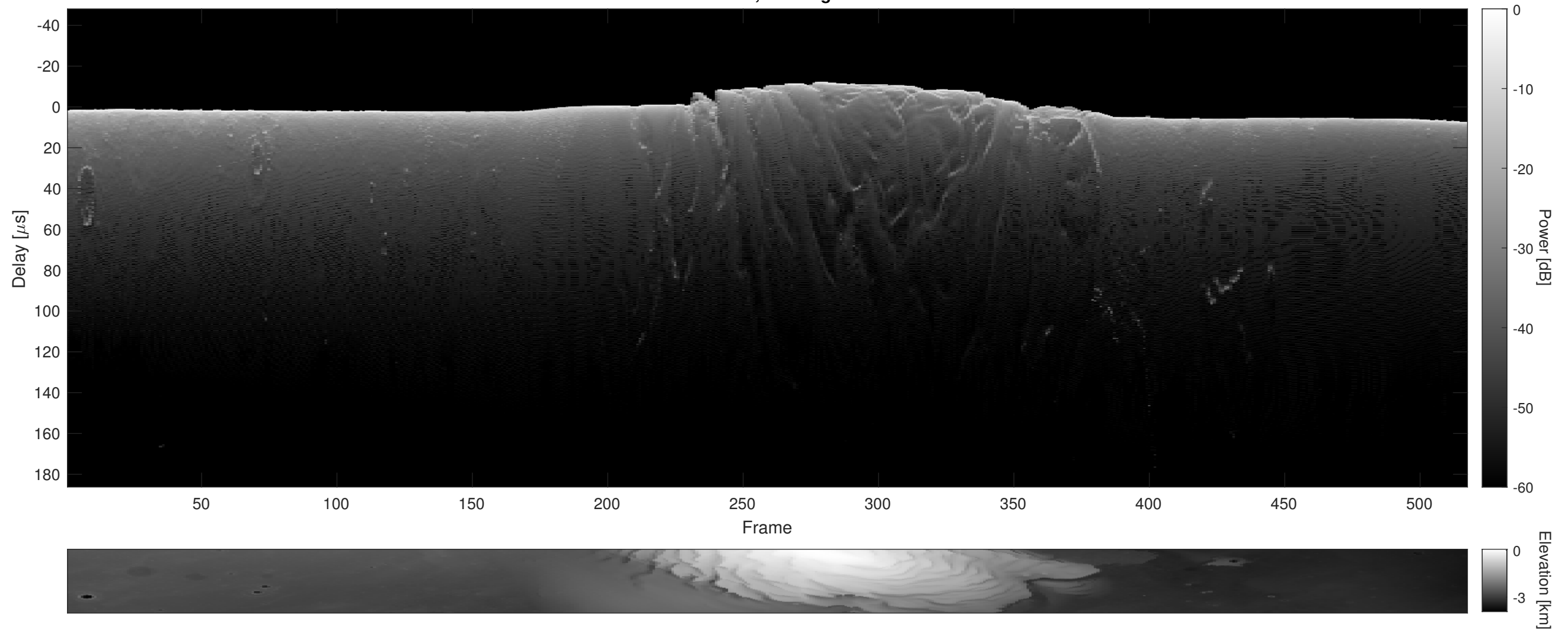
Orbit 5462, Cluttergram
