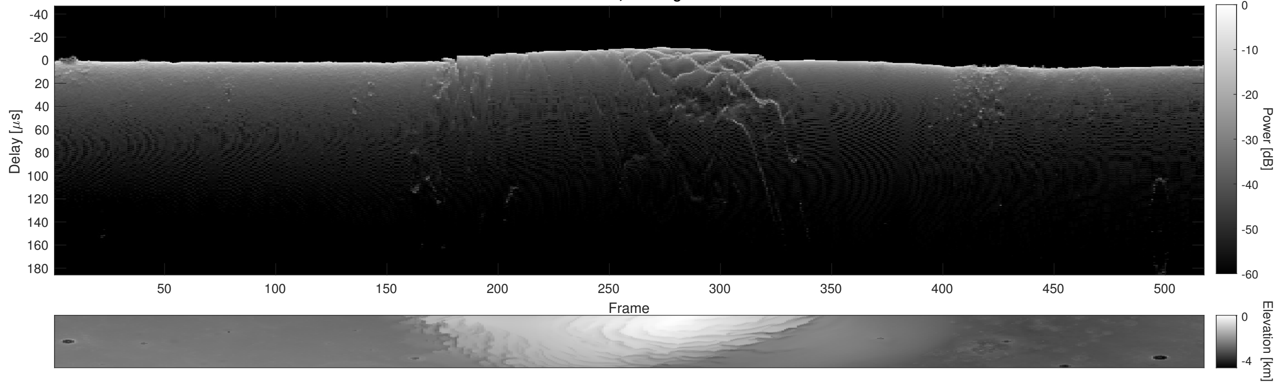
Orbit 5463, Cluttergram
