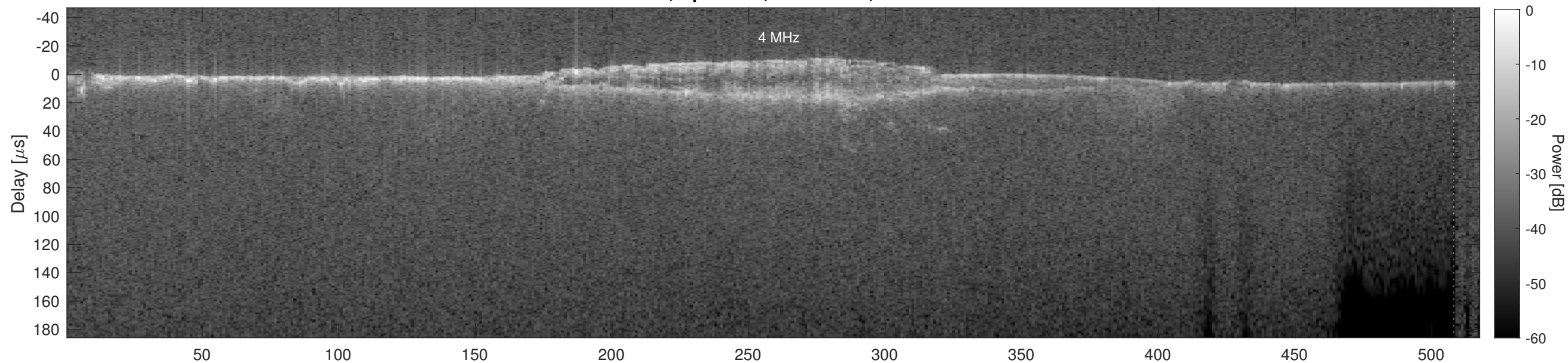
Orbit 5463, Cluttergram
