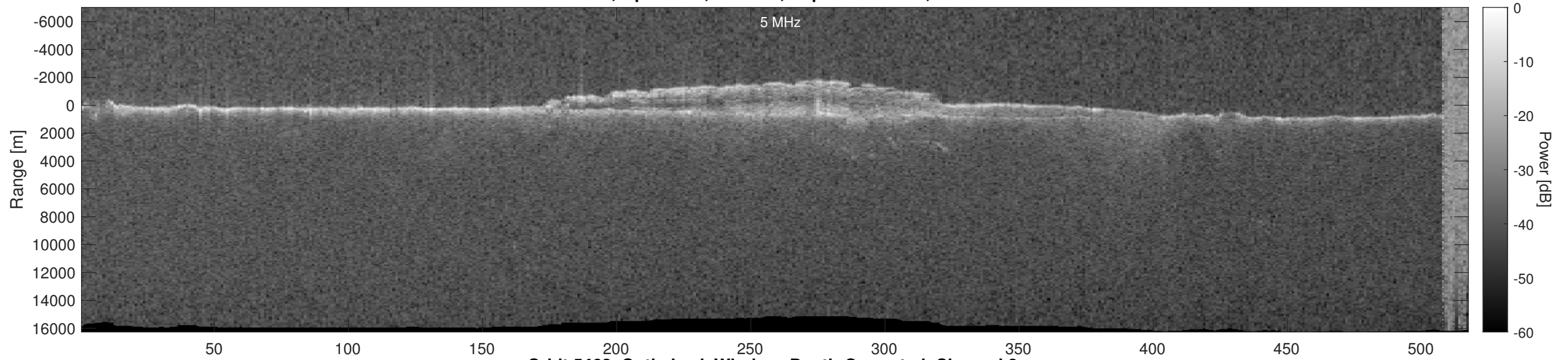
Orbit 5463, Optimized, Window, Depth-Corrected, Channel 2
