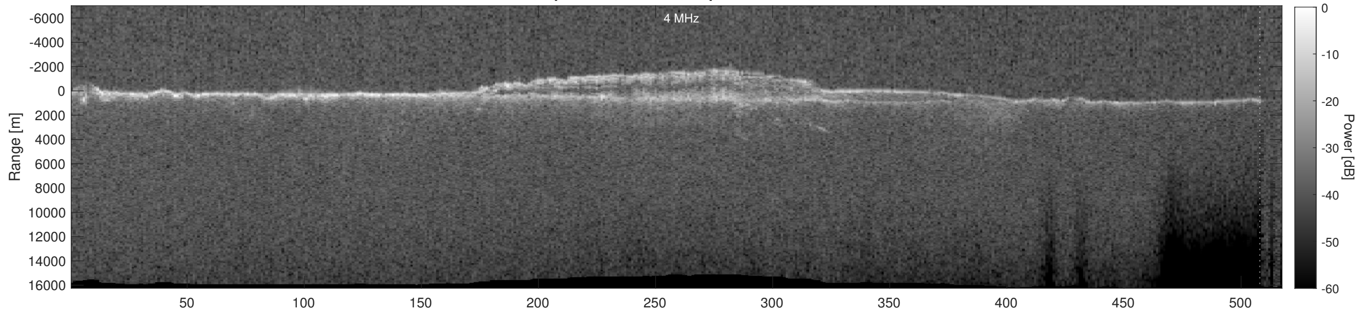
Orbit 5463, Depth-Corrected Cluttergram
