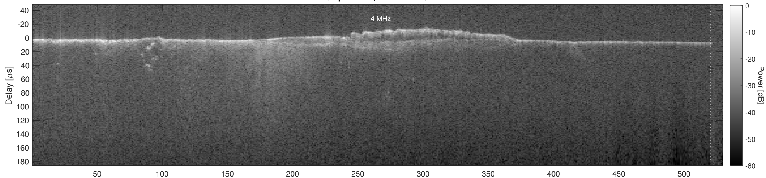
Orbit 5469, Cluttergram
