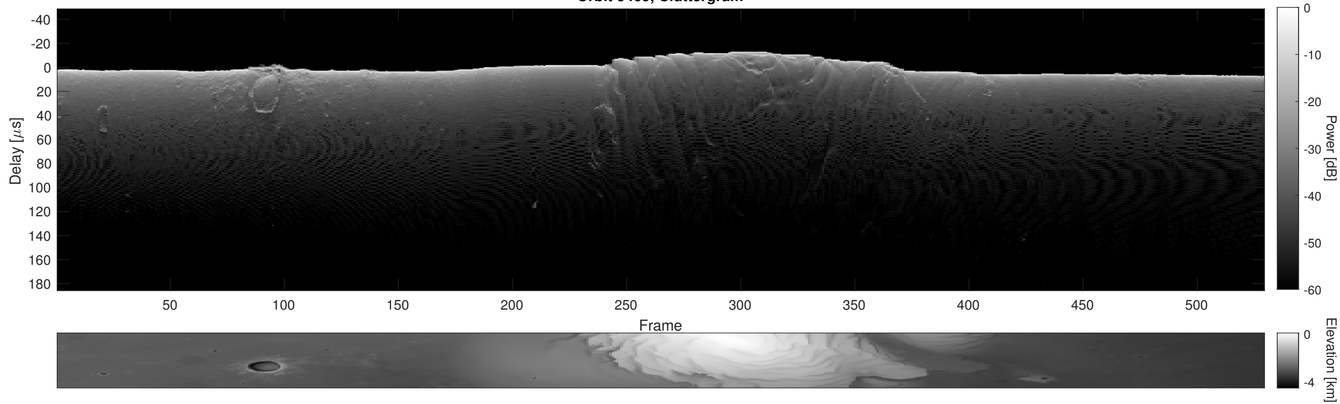
Orbit 5469, Cluttergram
