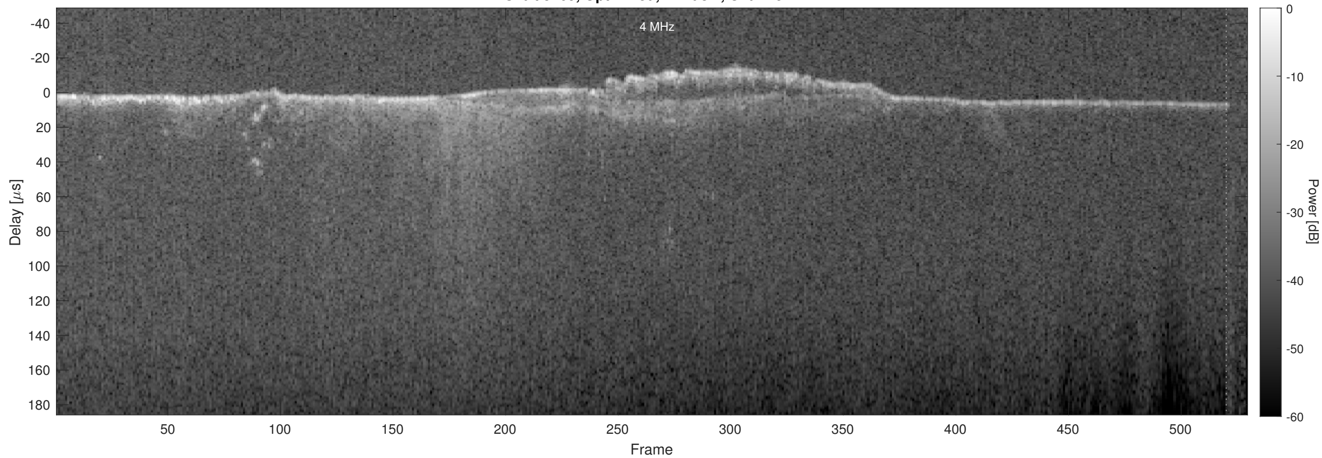
Orbit 5469, Optimized, Window, Channel 2
