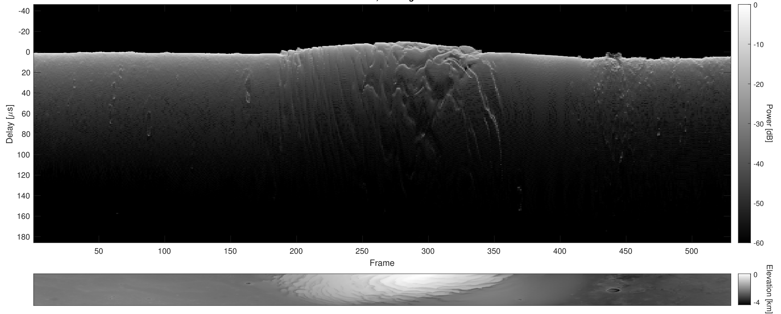
Orbit 5470, Cluttergram
