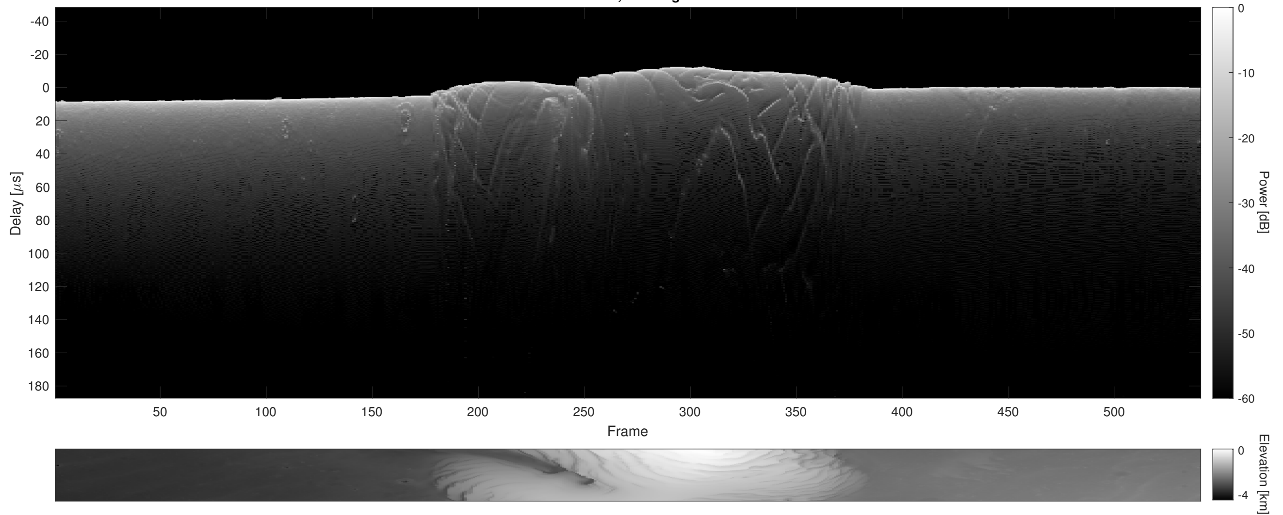
Orbit 5471, Cluttergram
