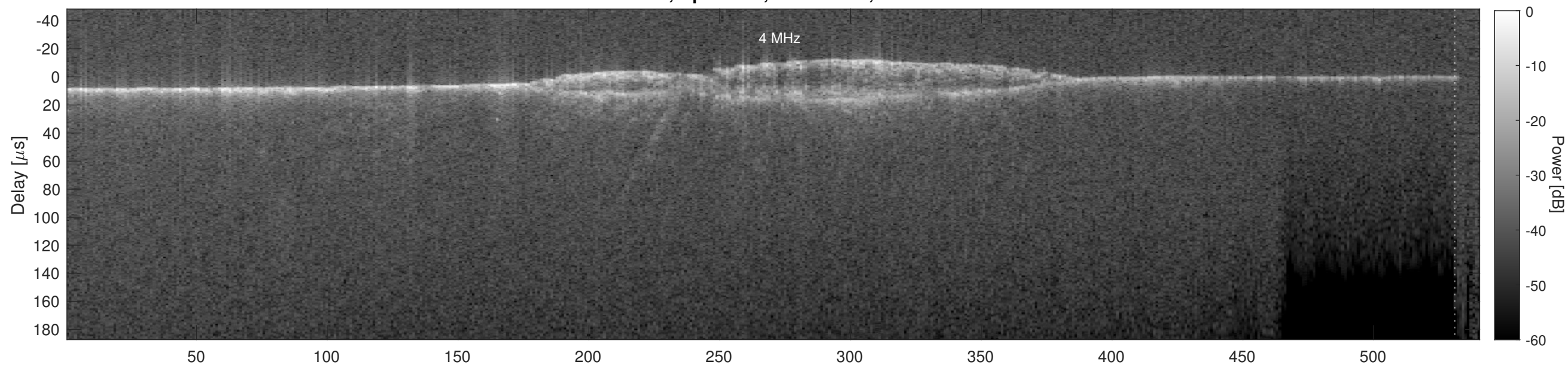
Orbit 5471, Cluttergram
