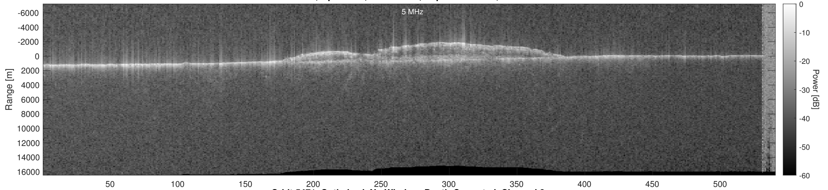
Orbit 5471, Optimized, No Window, Depth-Corrected, Channel 2
