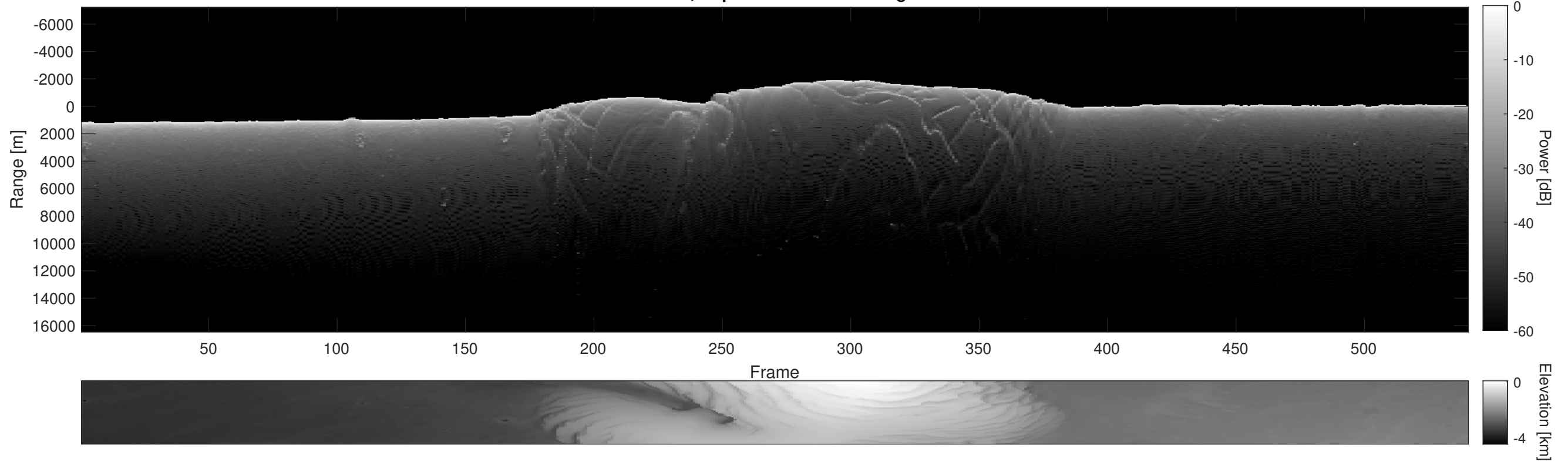
Orbit 5471, Depth-Corrected Cluttergram
