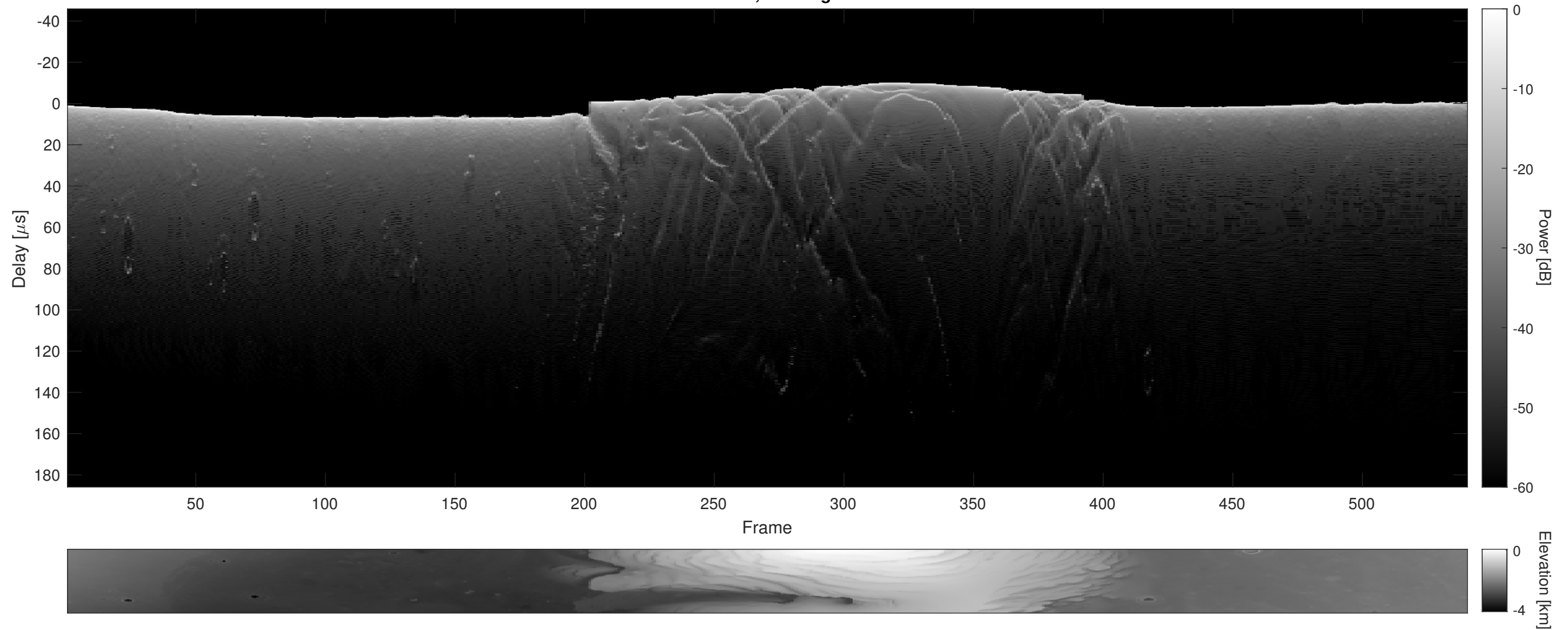
Orbit 5475, Cluttergram
