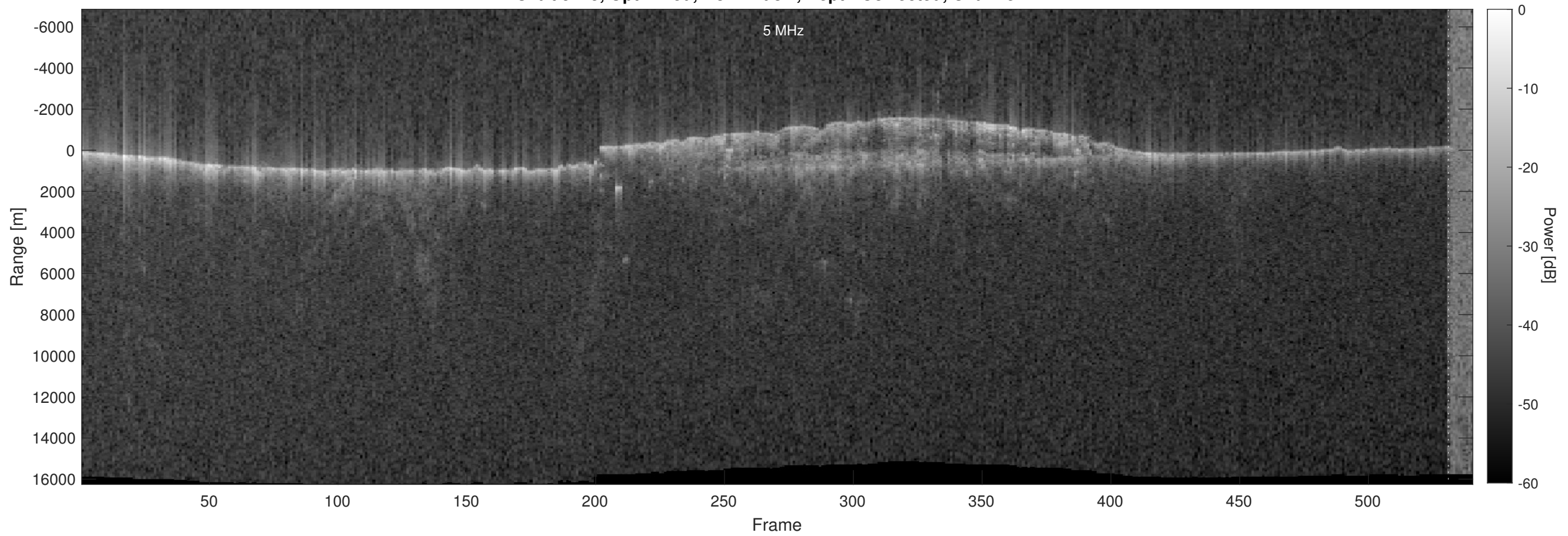
Orbit 5475, Optimized, No Window, Depth-Corrected, Channel 2
