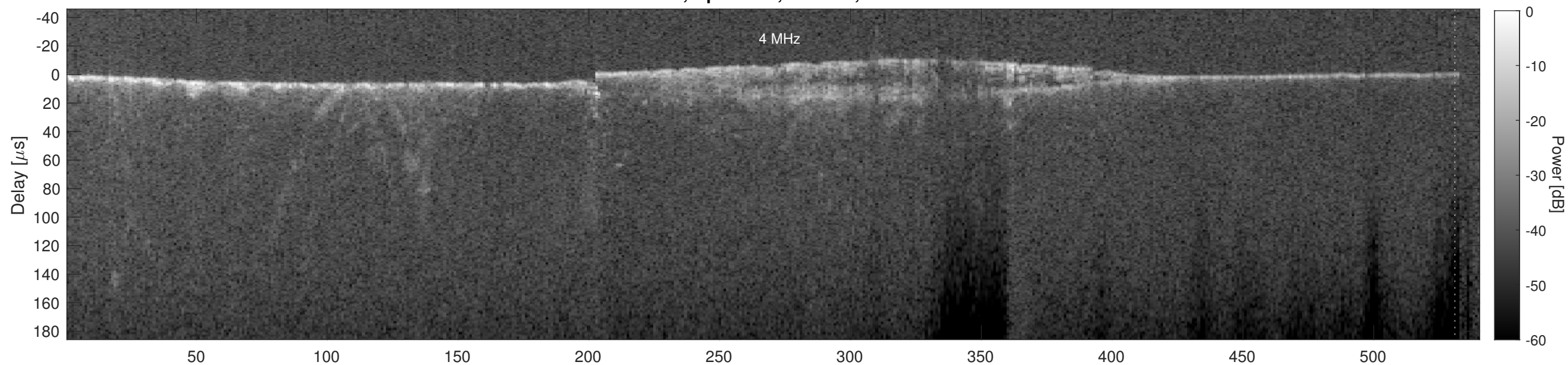
Orbit 5475, Cluttergram
