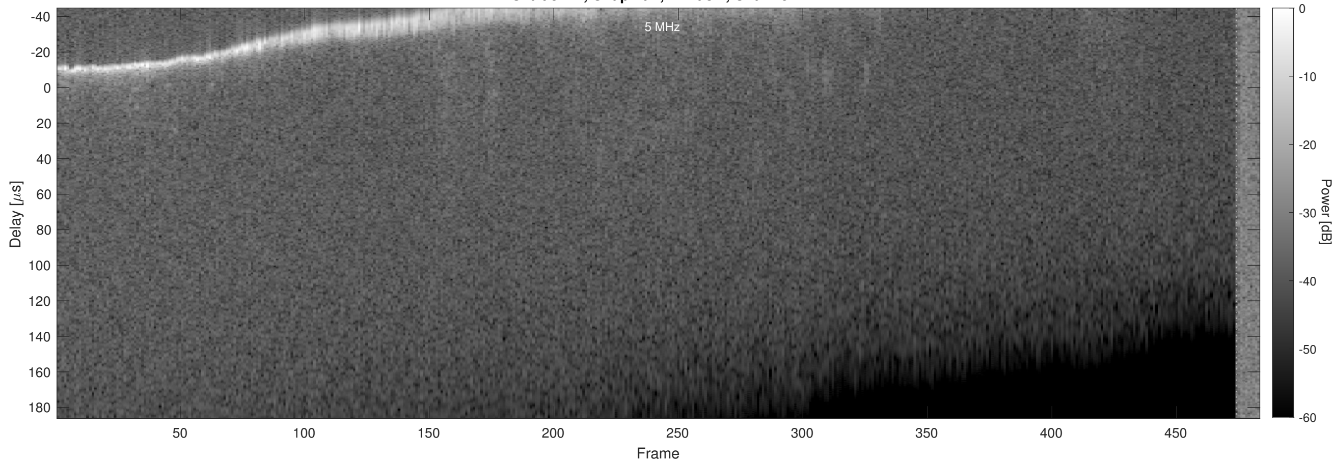
Orbit 5477, Chapman, Window, Channel 2
