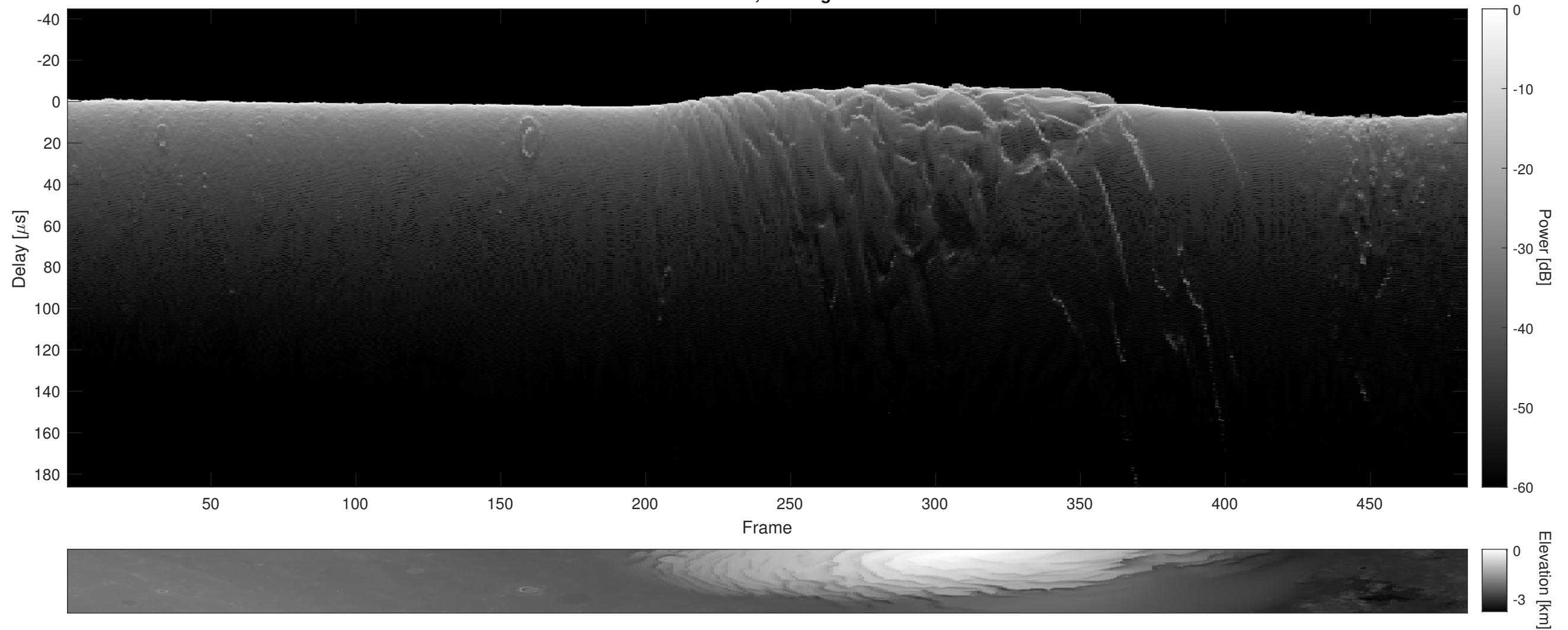
Orbit 5477, Cluttergram
