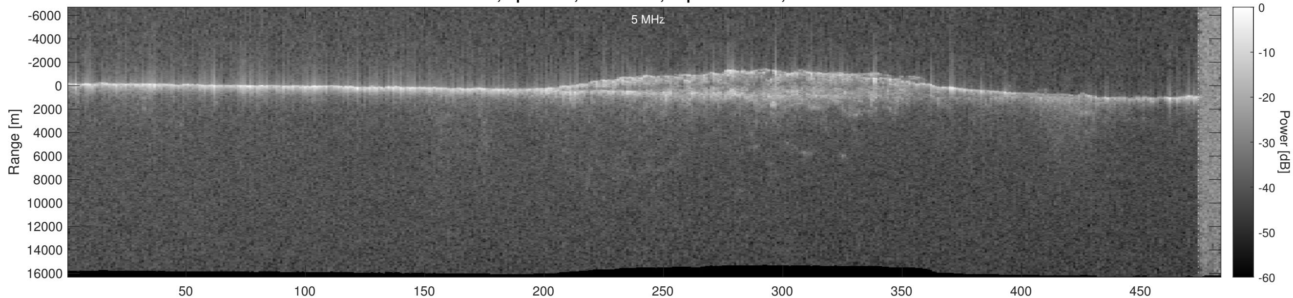
Orbit 5477, Optimized, No Window, Depth-Corrected, Channel 2
