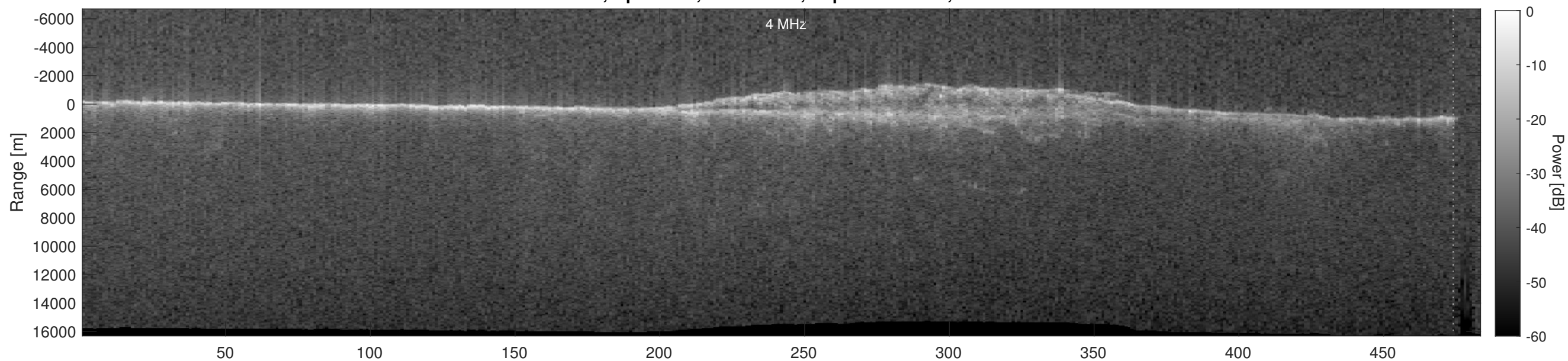
Orbit 5477, Depth-Corrected Cluttergram
