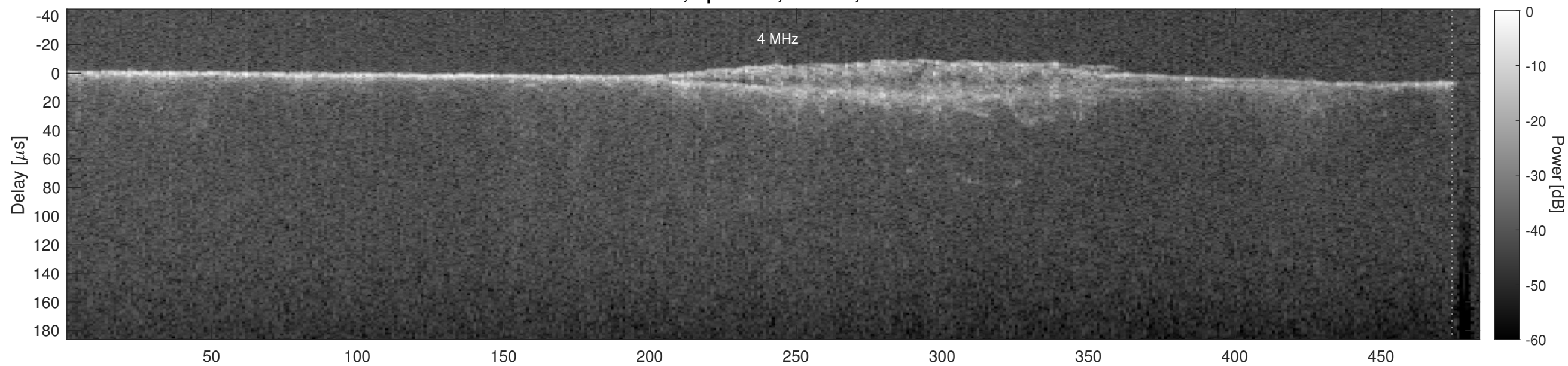
Orbit 5477, Cluttergram
