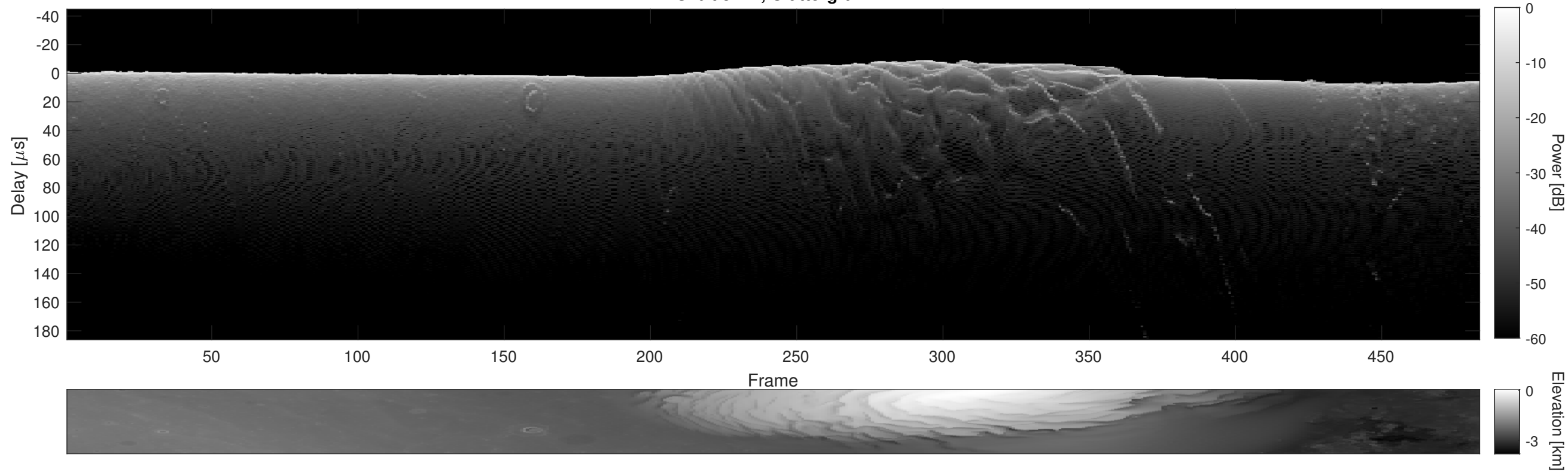
Orbit 5477, Cluttergram
