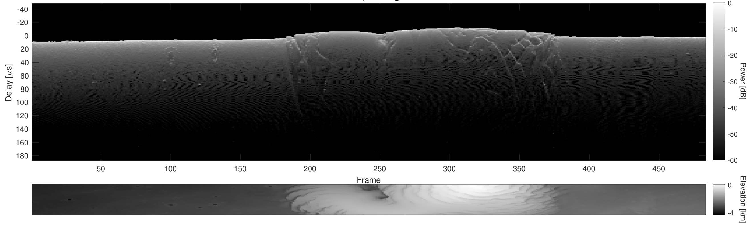
Orbit 5478, Cluttergram
