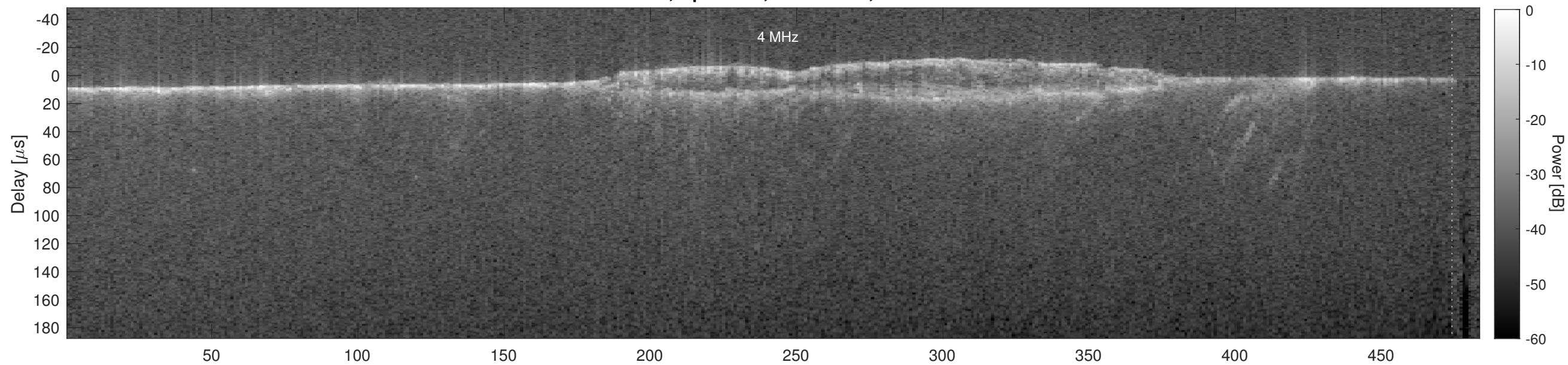
Orbit 5478, Cluttergram
