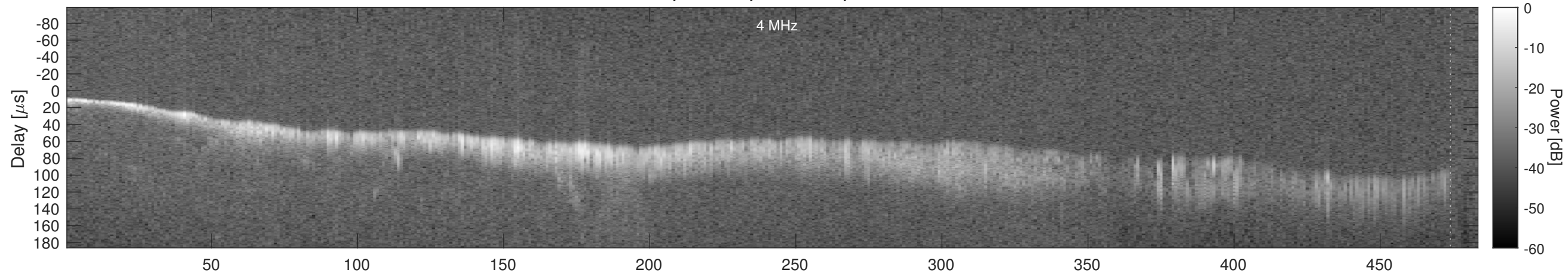
Orbit 5479, Window, Channel 2, Chapman
