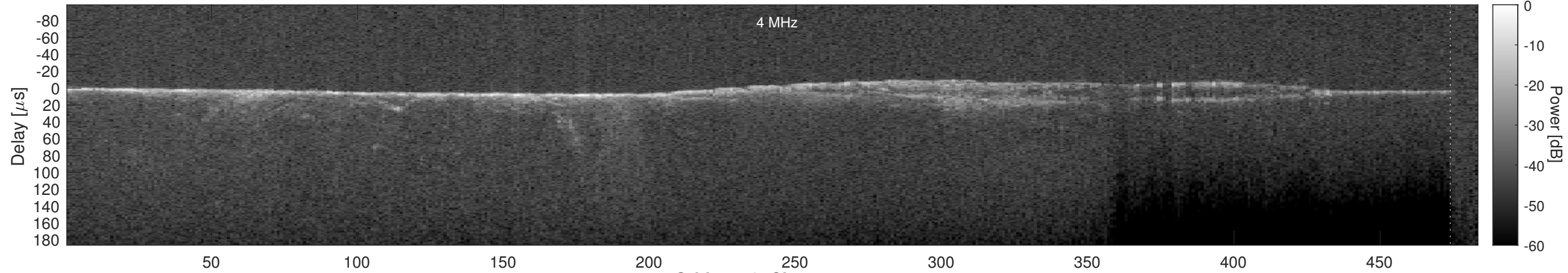
Orbit 5479, Cluttergram
