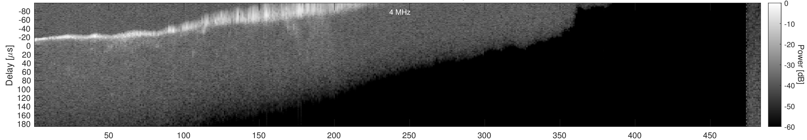
Orbit 5479, Window, Channel 2, Optimized
