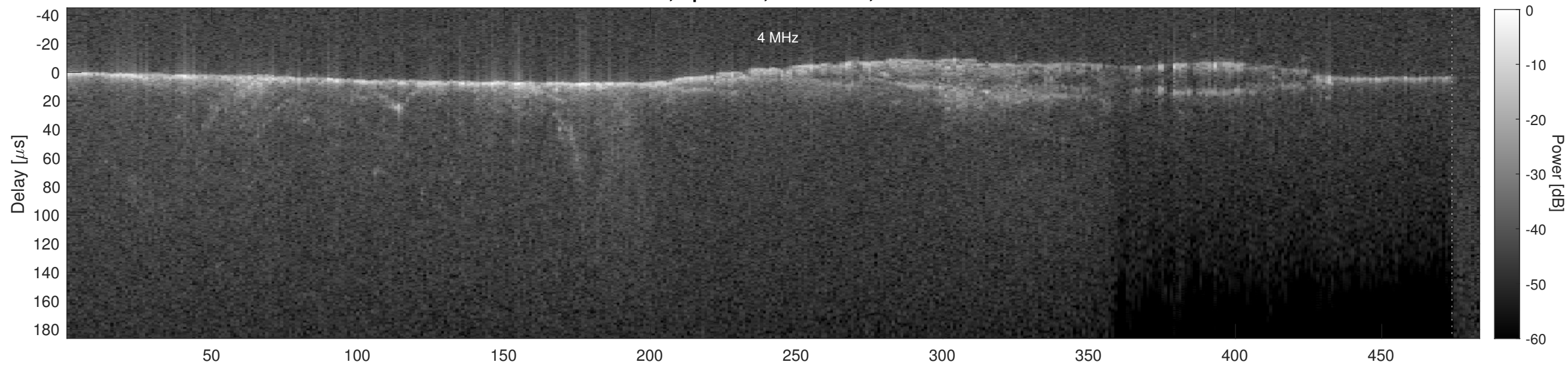
Orbit 5479, Cluttergram
