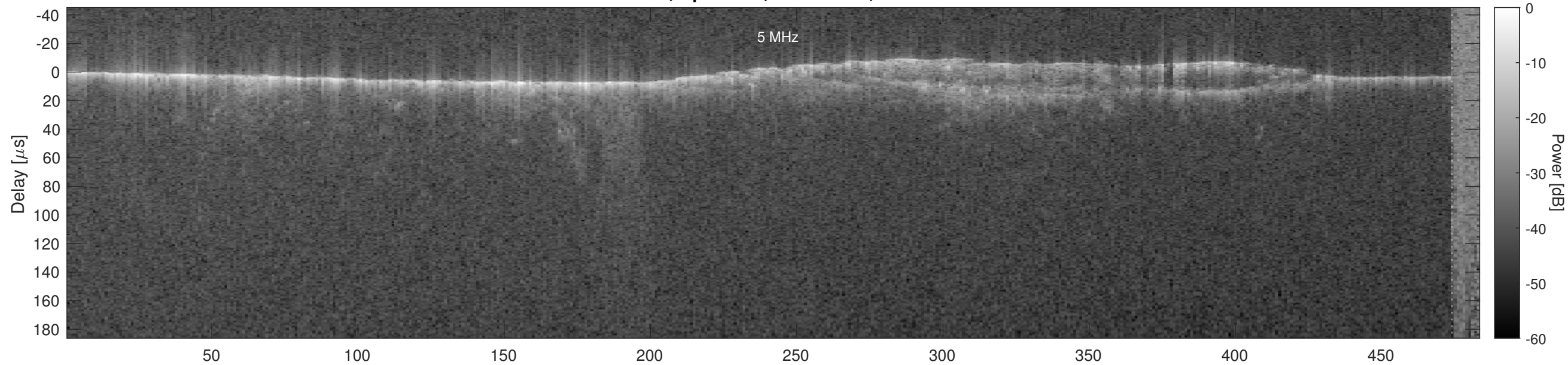
Orbit 5479, Optimized, No Window, Channel 2
