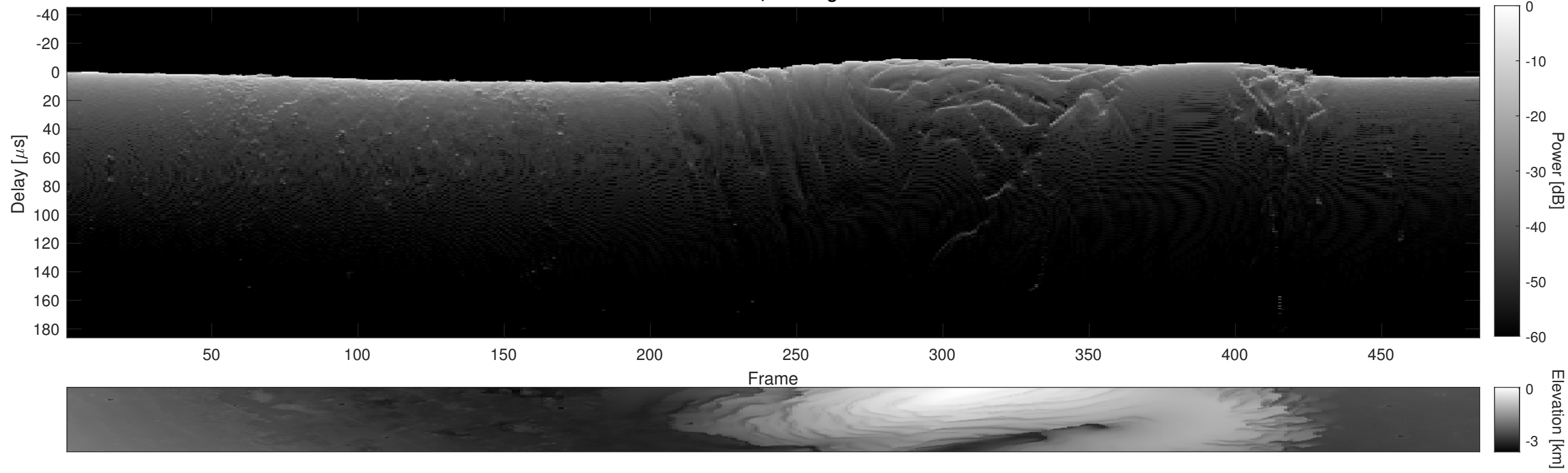
Orbit 5479, Cluttergram
