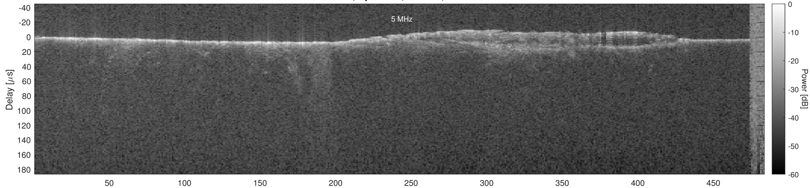
Orbit 5479, Optimized, Window, Channel 2
