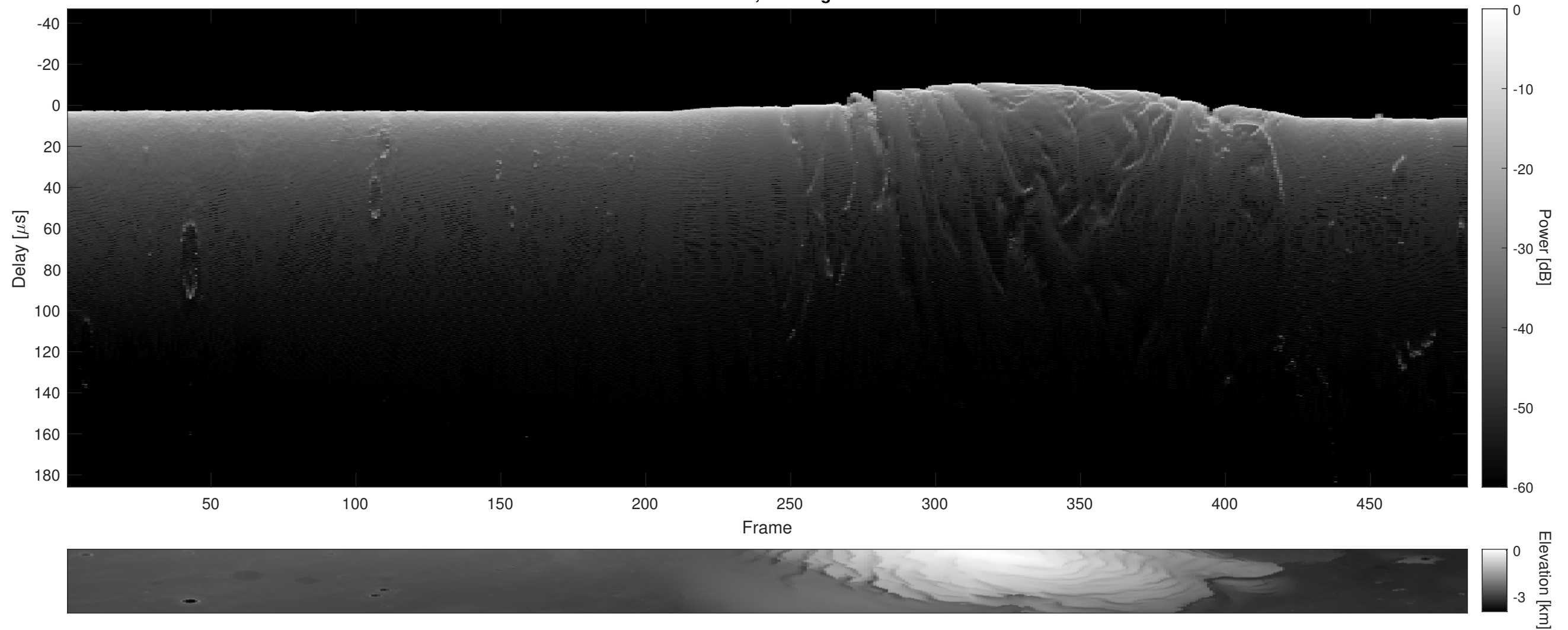
Orbit 5480, Cluttergram
