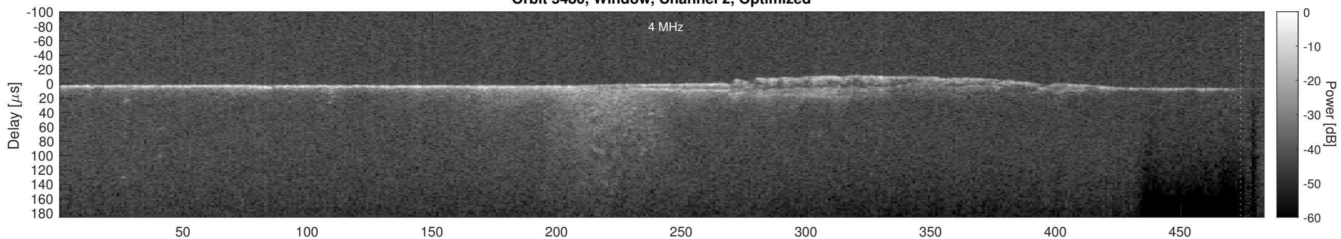
Orbit 5480, Cluttergram
