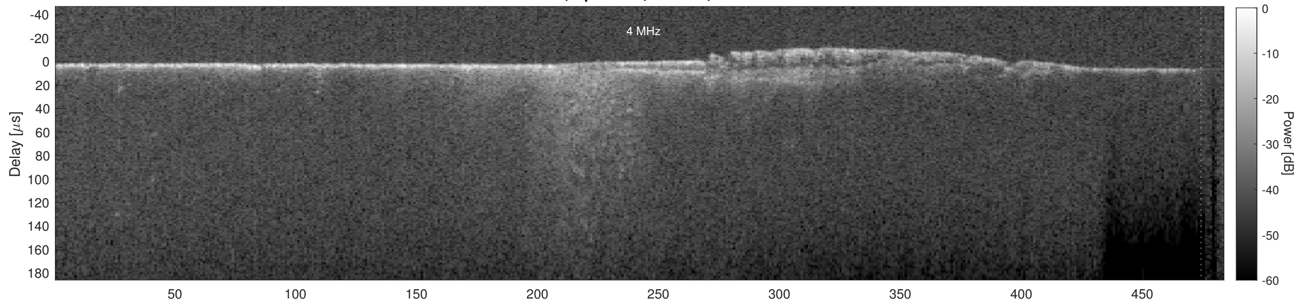
Orbit 5480, Cluttergram
