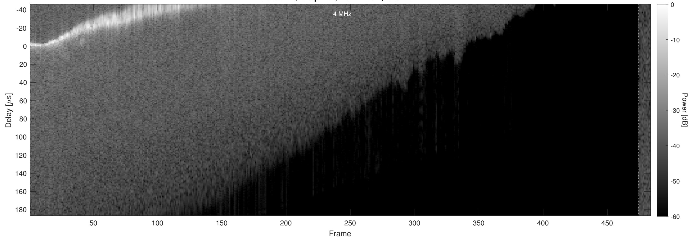
Orbit 5481, Chapman, No Window, Channel 2
