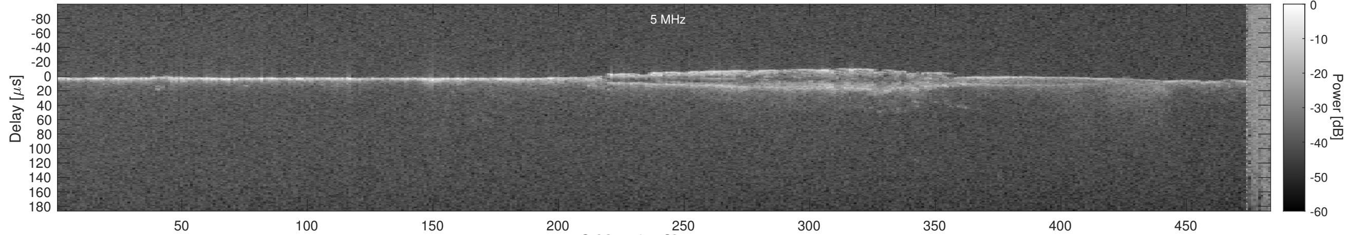
Orbit 5481, Cluttergram
