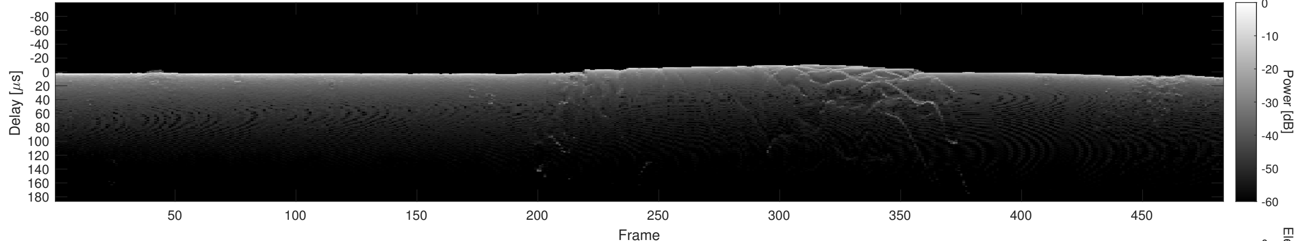
Orbit 5481, Cluttergram
